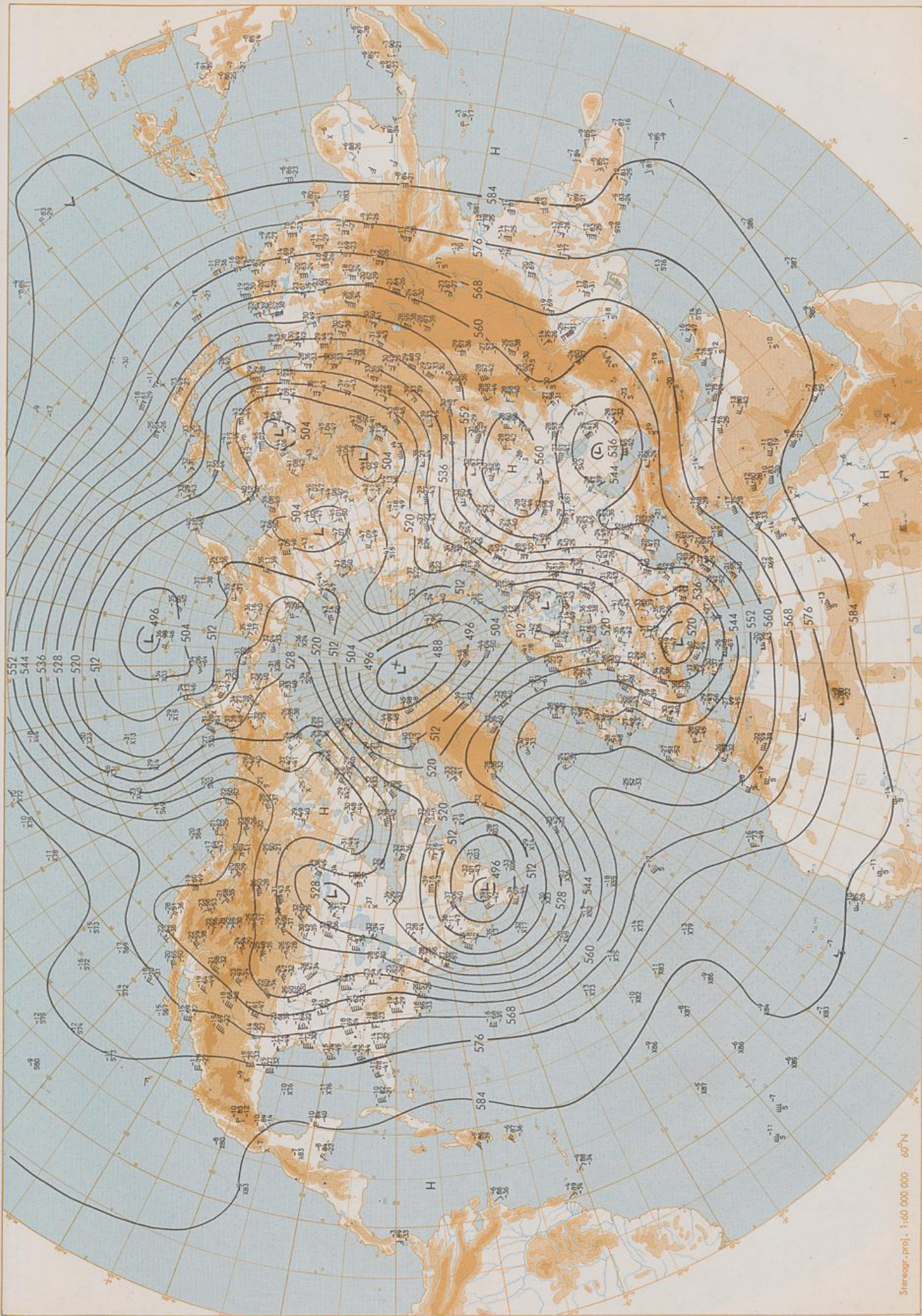
500 hPa 00 UTC
