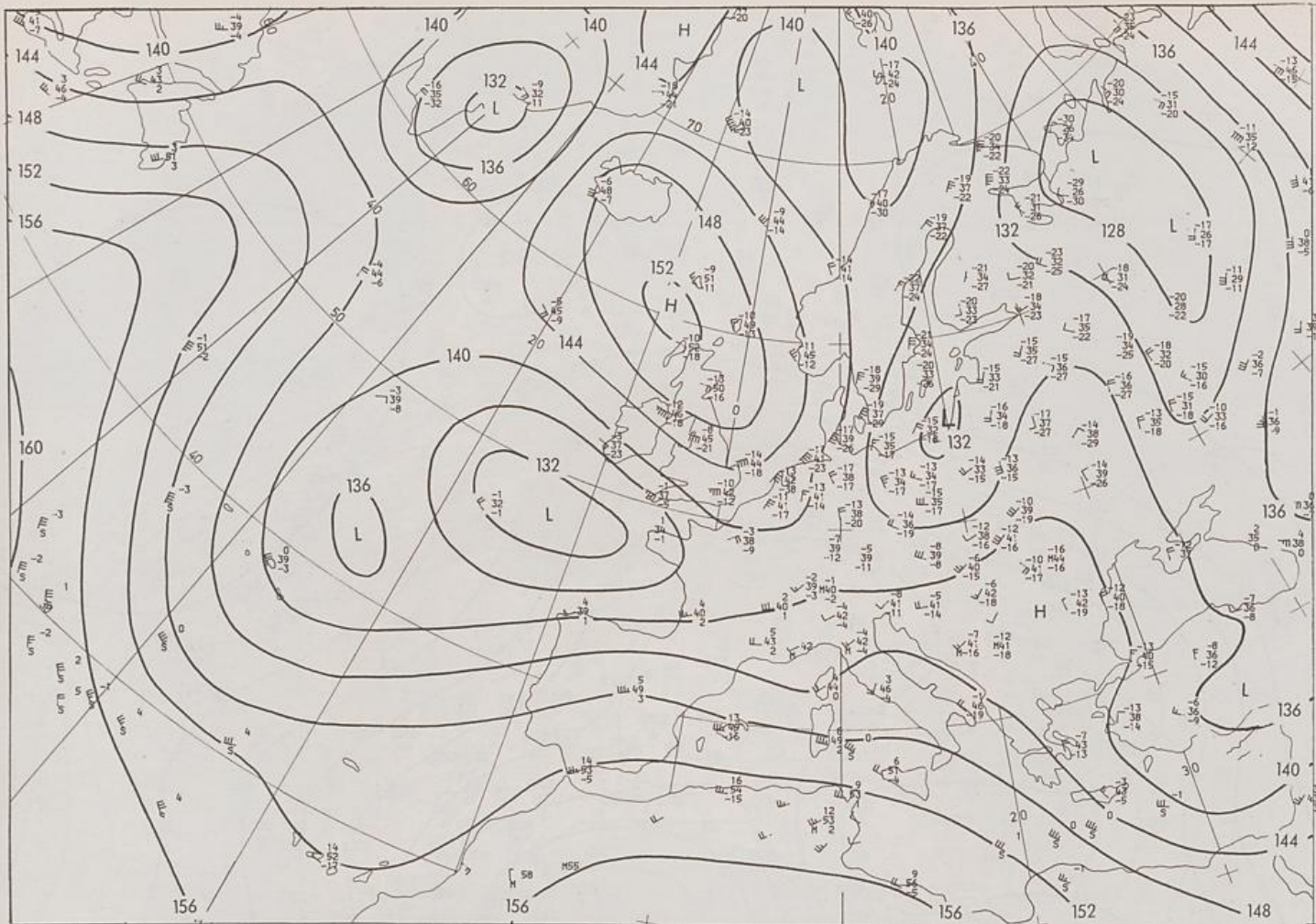
850 hPa 00 UTC
