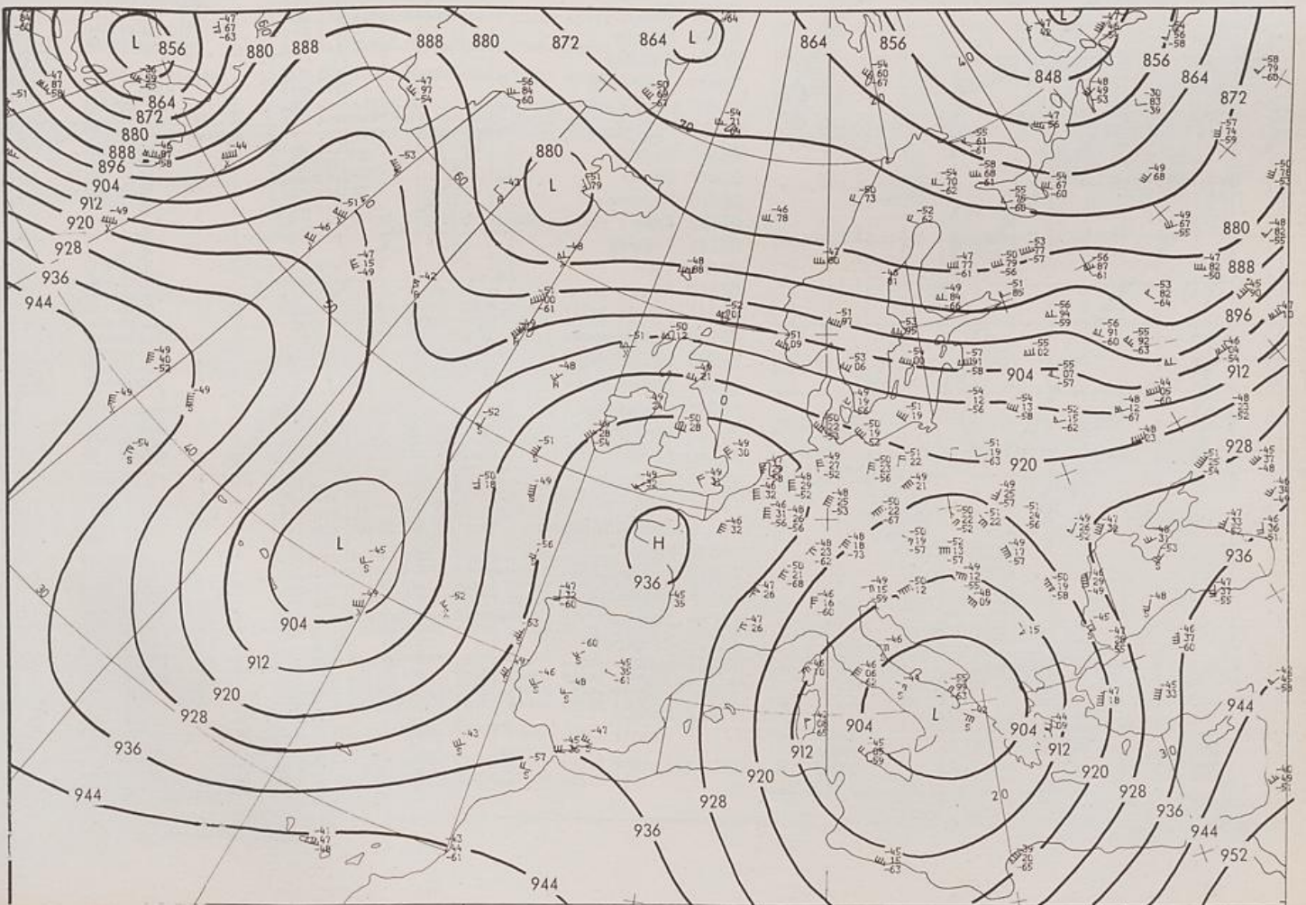
300 hPa 00 UTC
