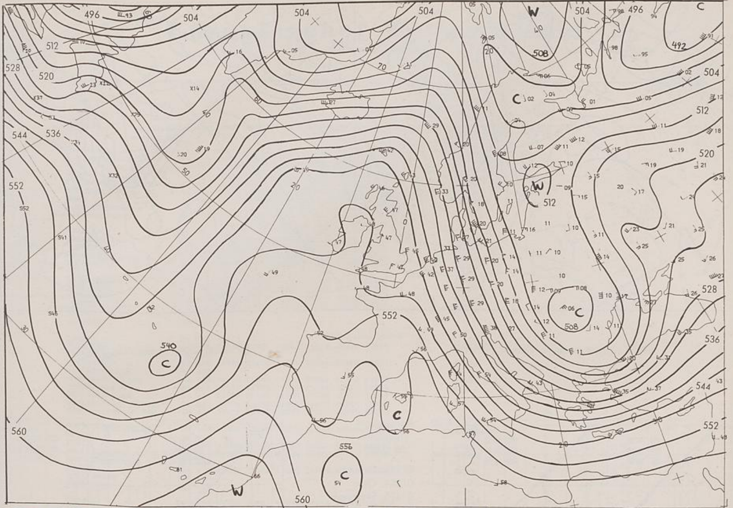
500/1000 hPa 00 UTC
