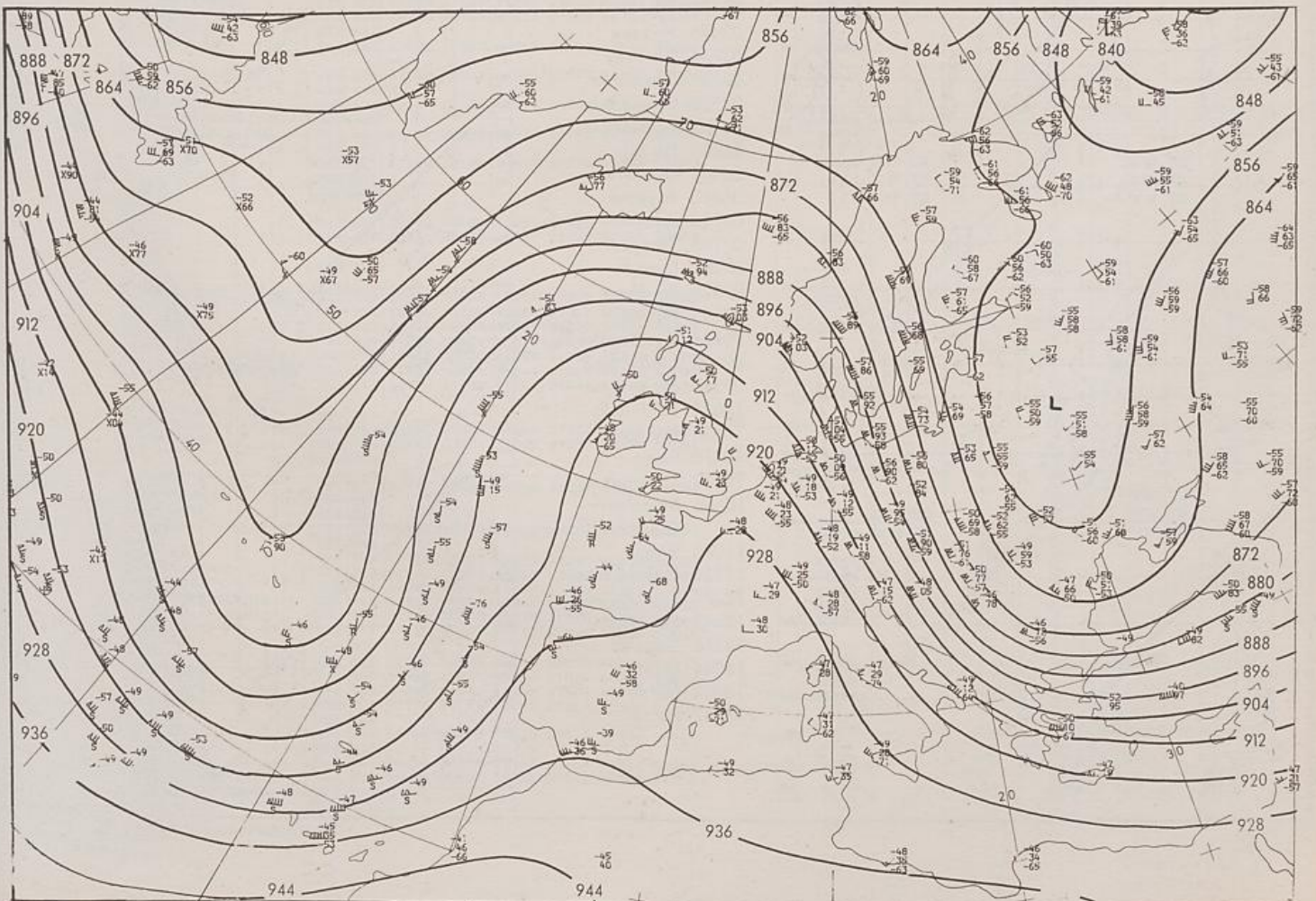
300 hPa 00 UTC
