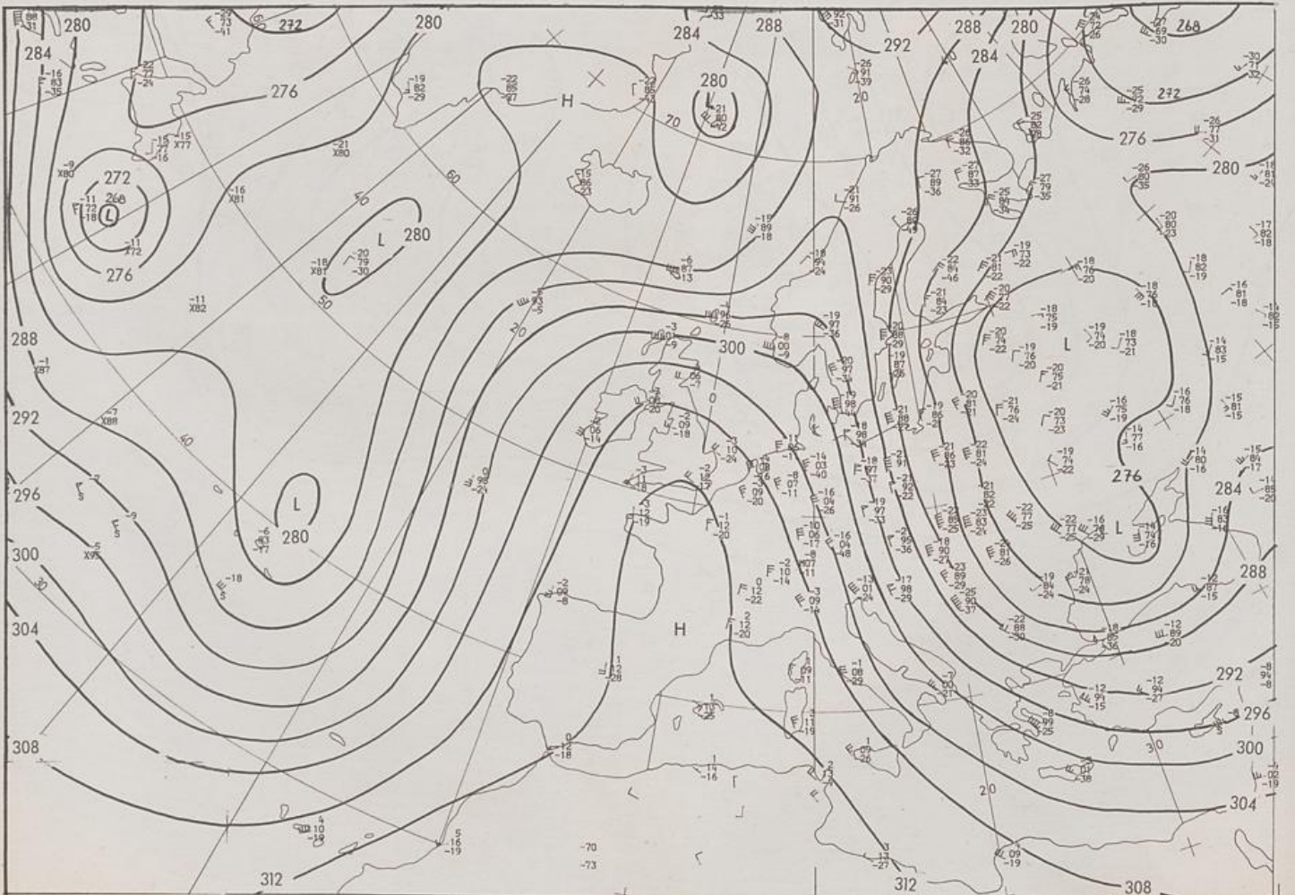
700 hPa 00 UTC
