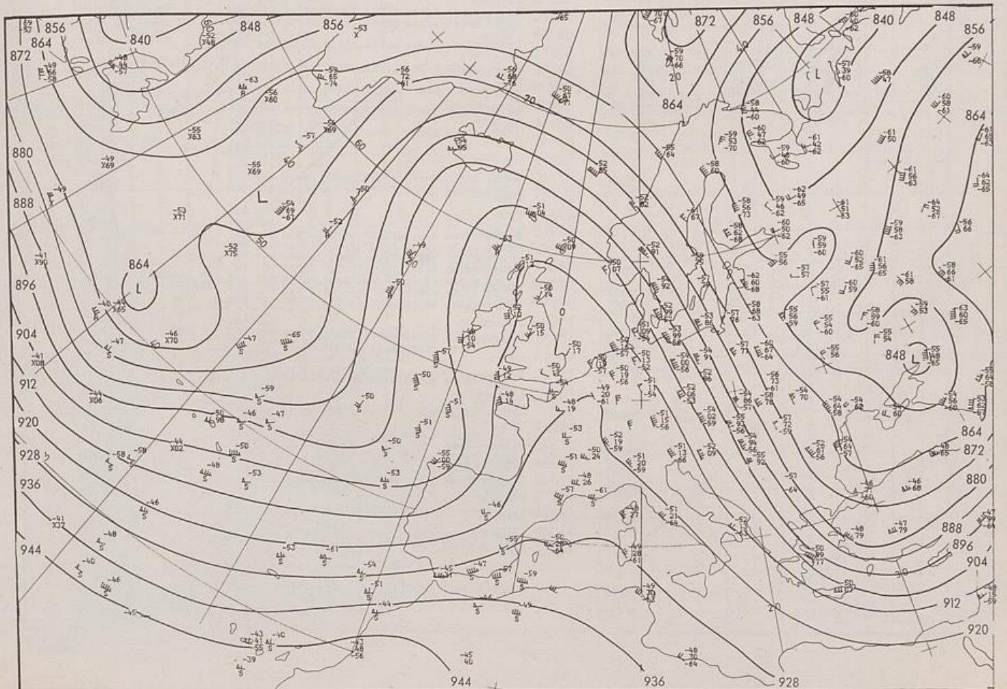
300 hPa 00 UTC
