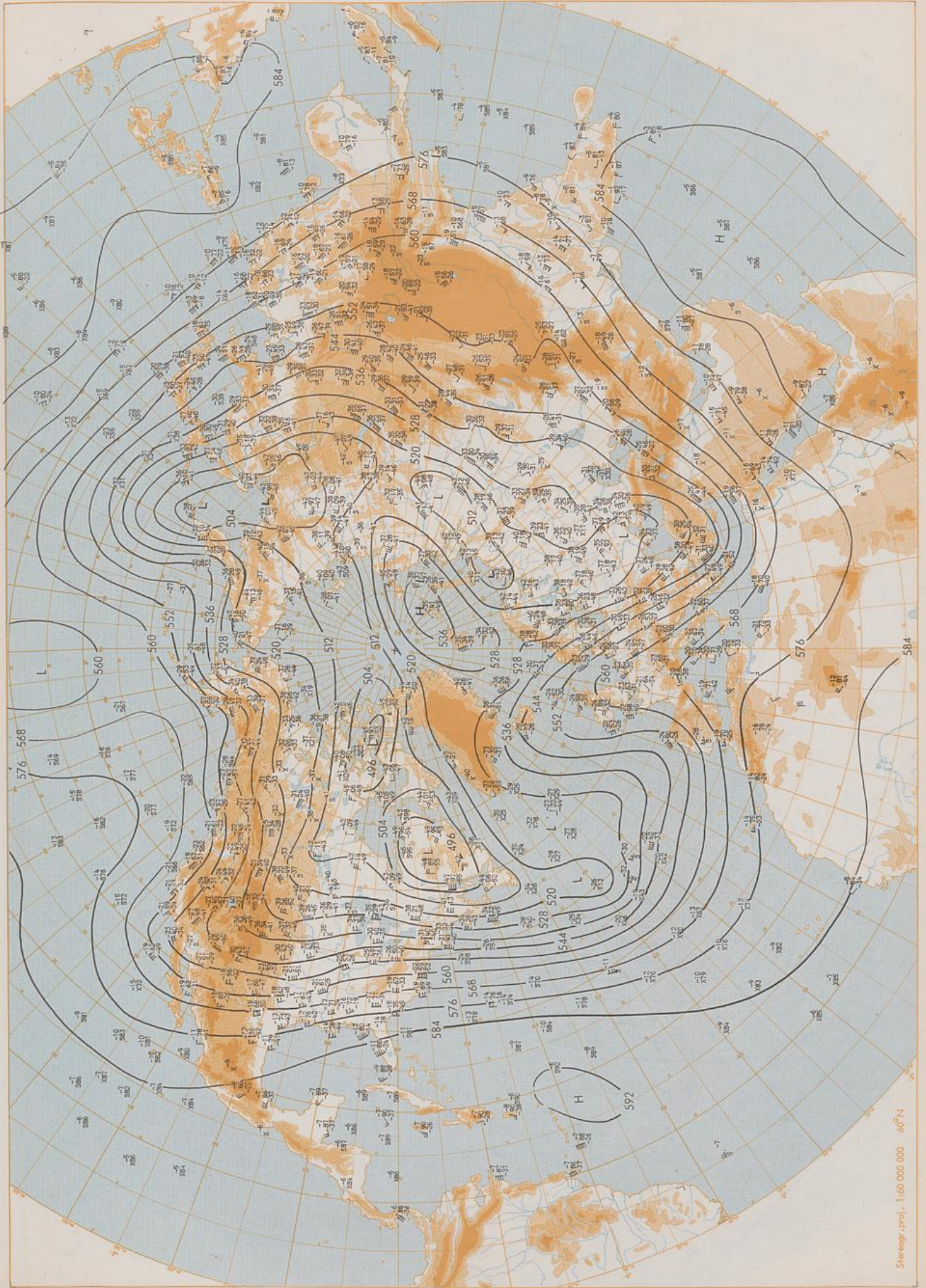
500 hPa 00 UTC
