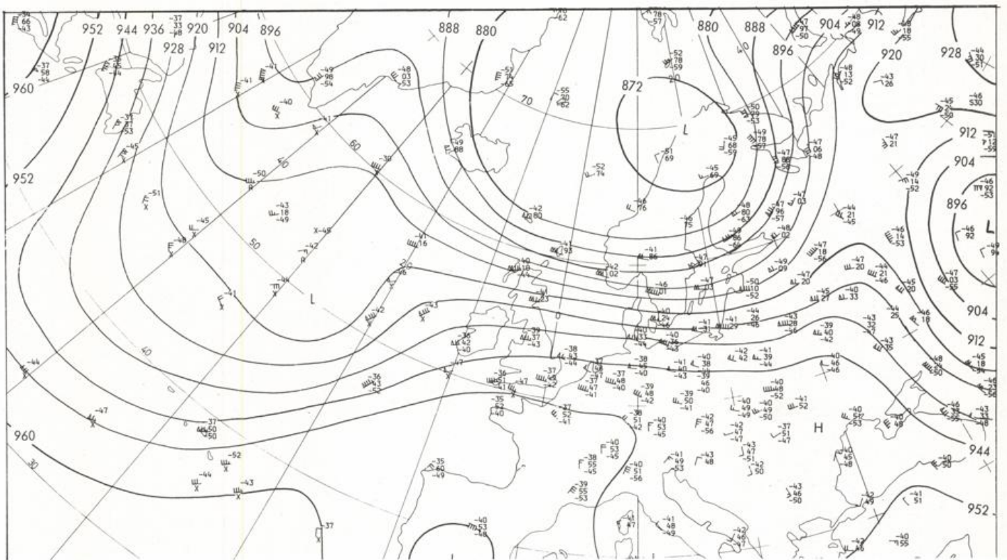
500/1000 hPa 00 UTC
