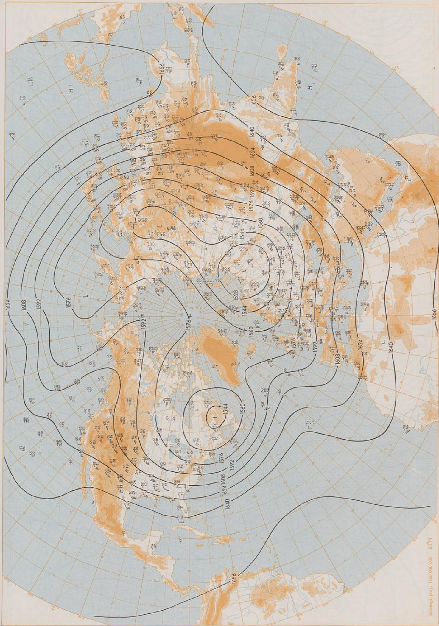
100 hPa 00 UTC
