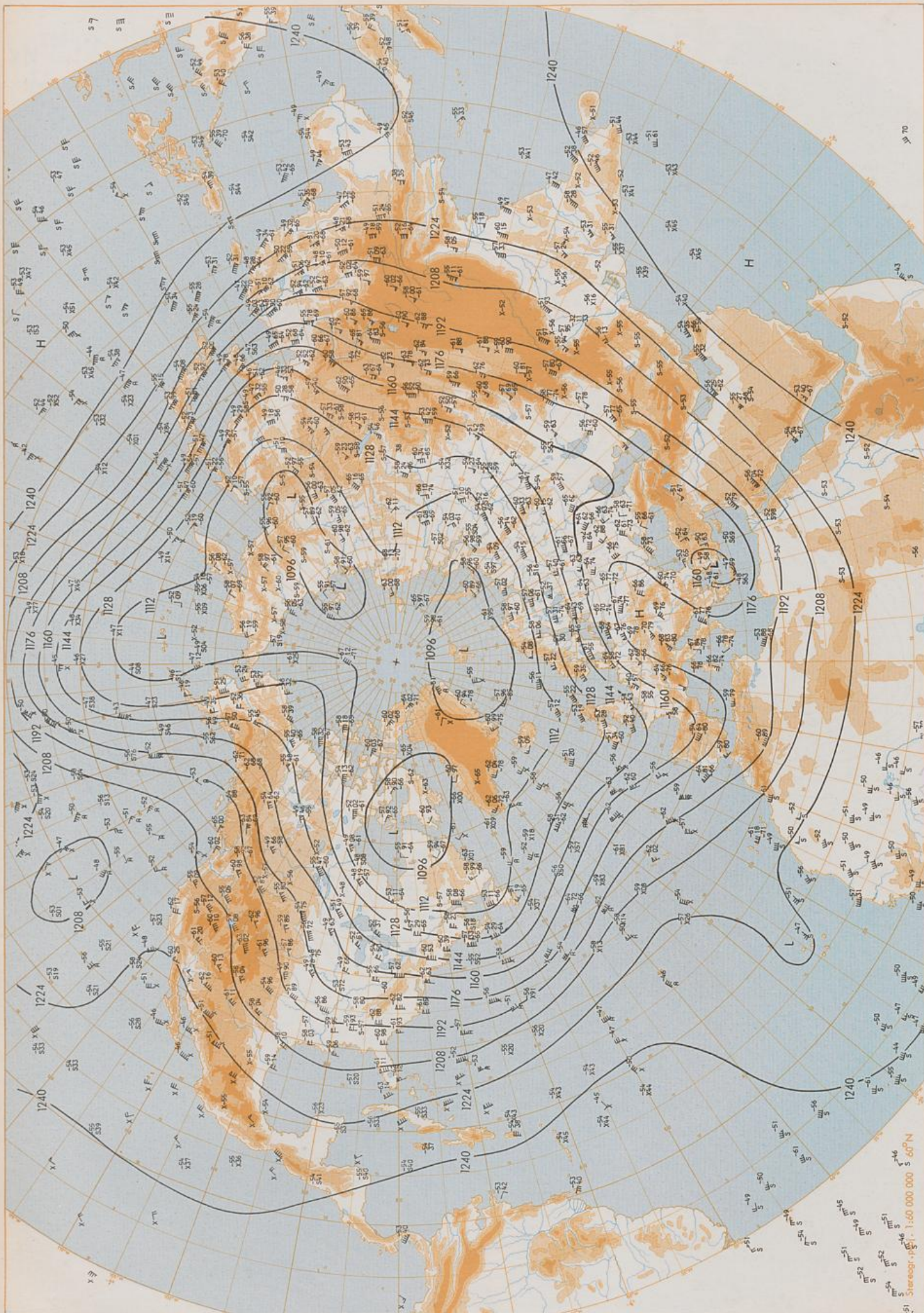
200 hPa 00 UTC
