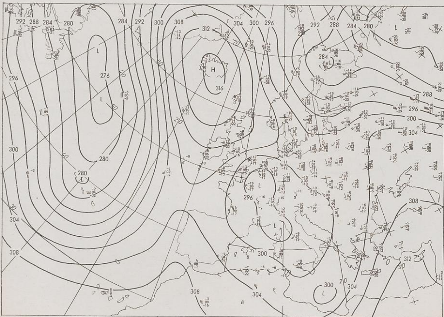
700 hPa 00 UTC
