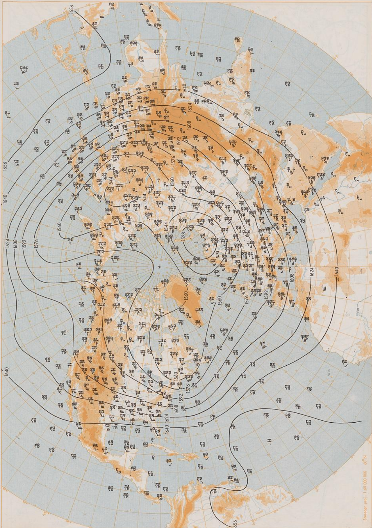
100 hPa 00 UTC
