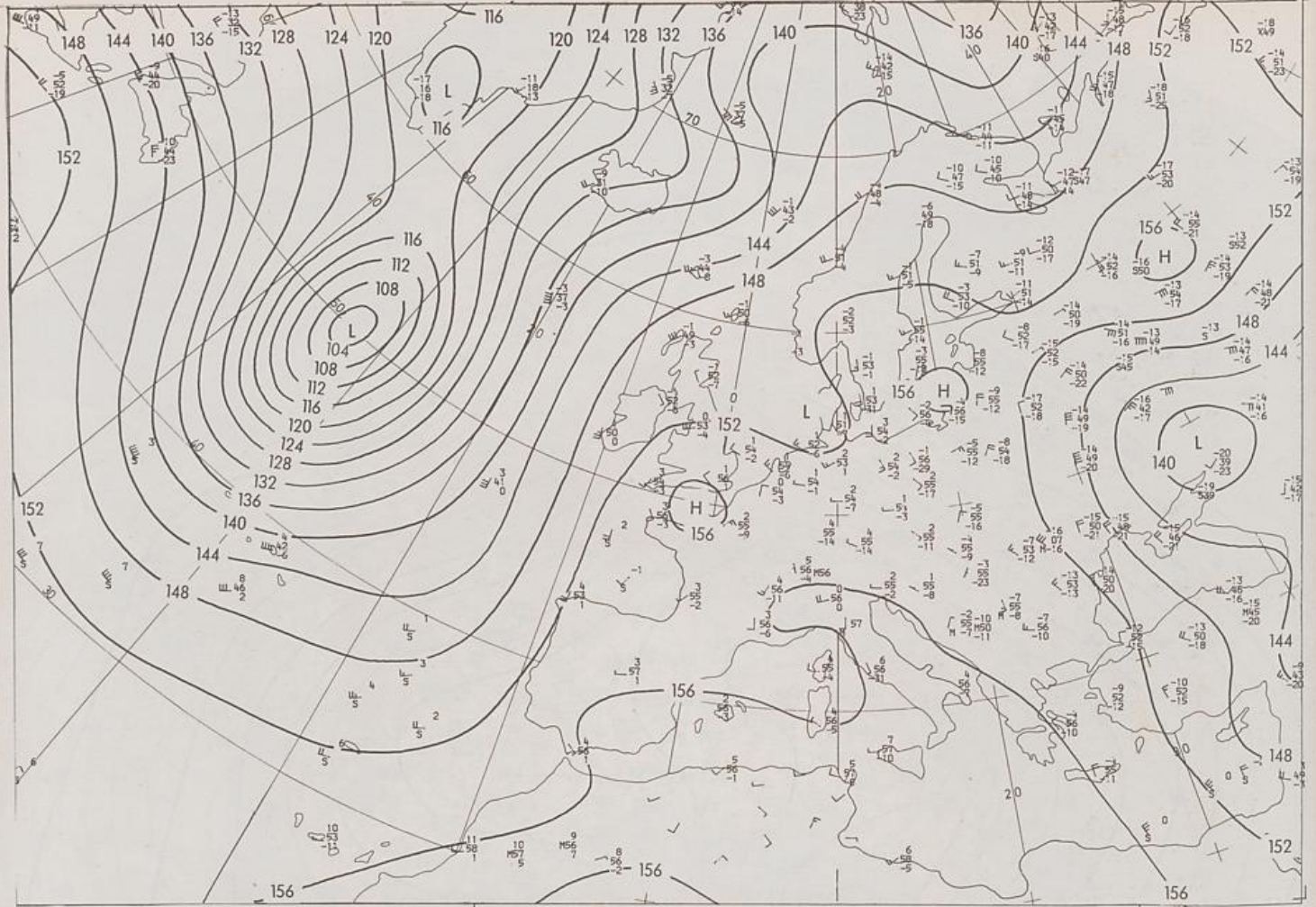
850 hPa 00 UTC
