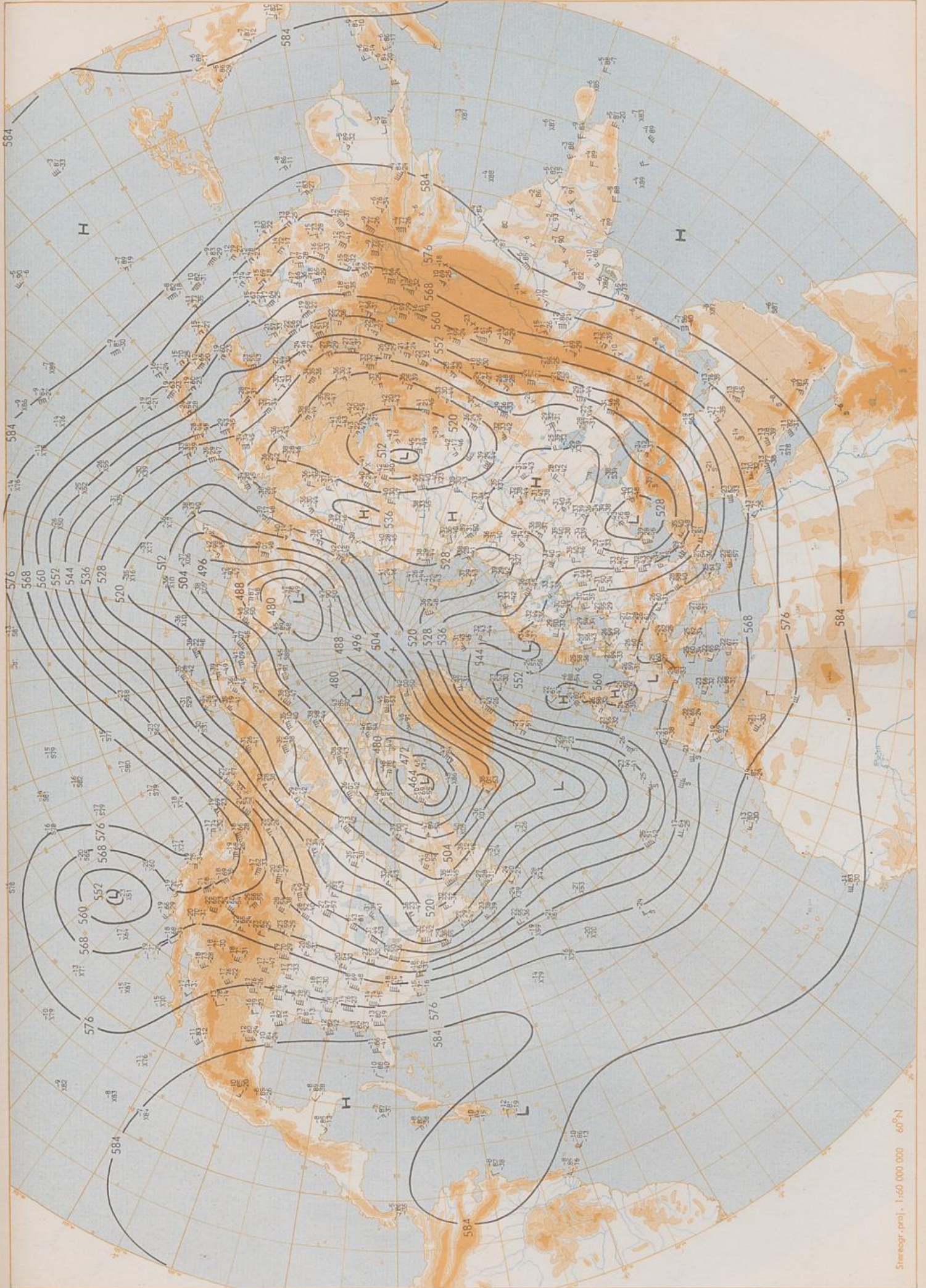
500 hPa 00 UTC
