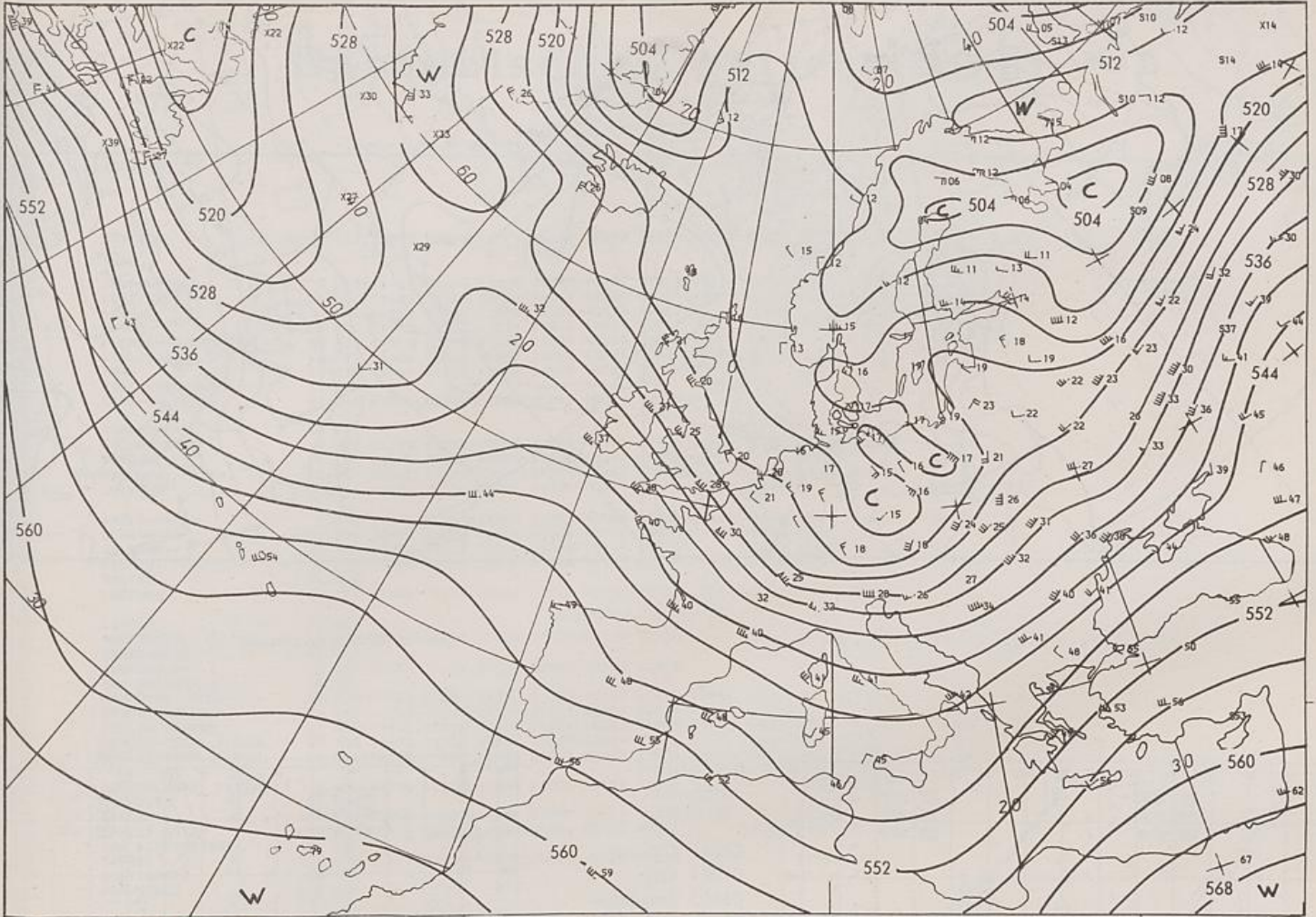
500/1000 hPa 00 UTC
