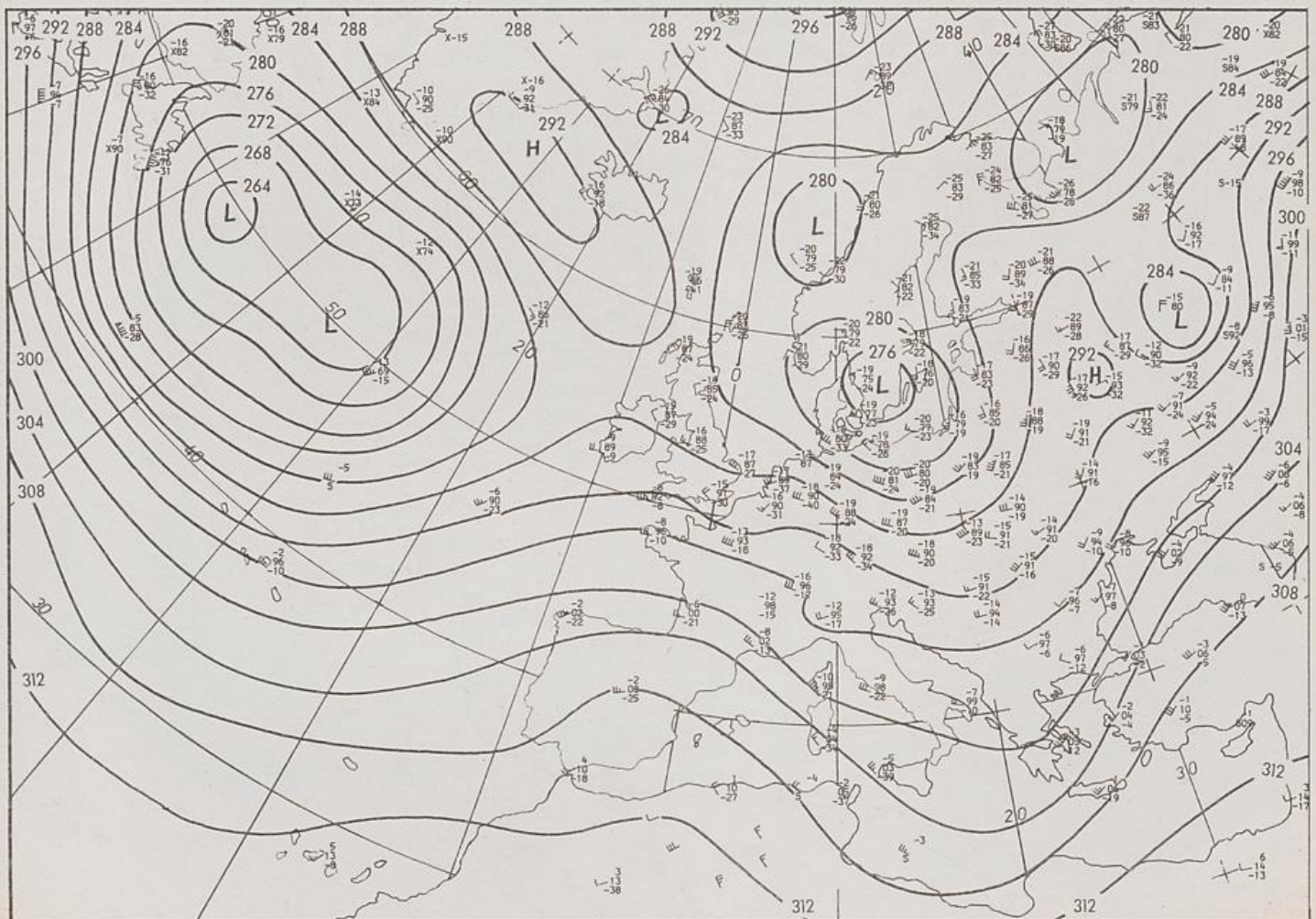
700 hPa 00 UTC
