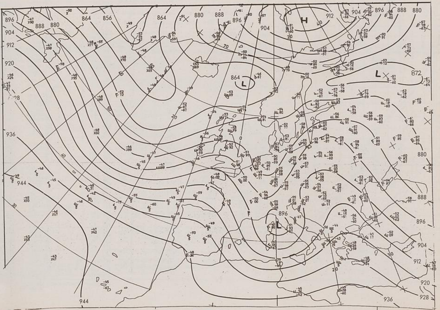
300 hPa 00 UTC
