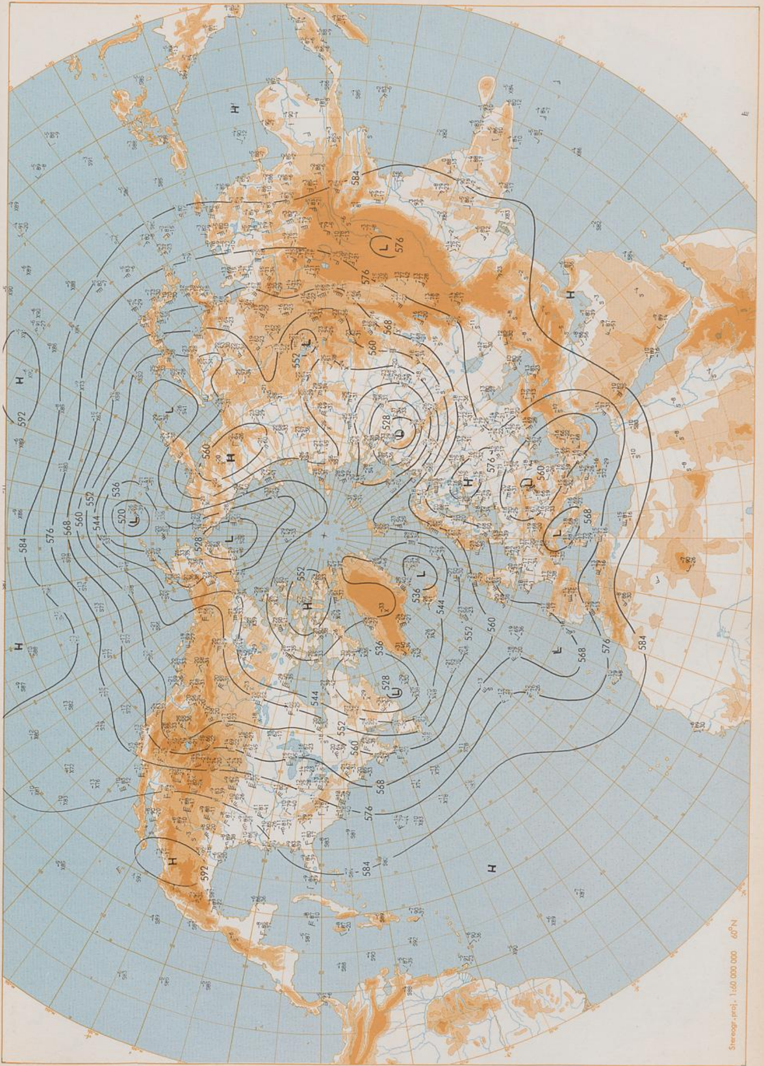
500 hPa 00 UTC
