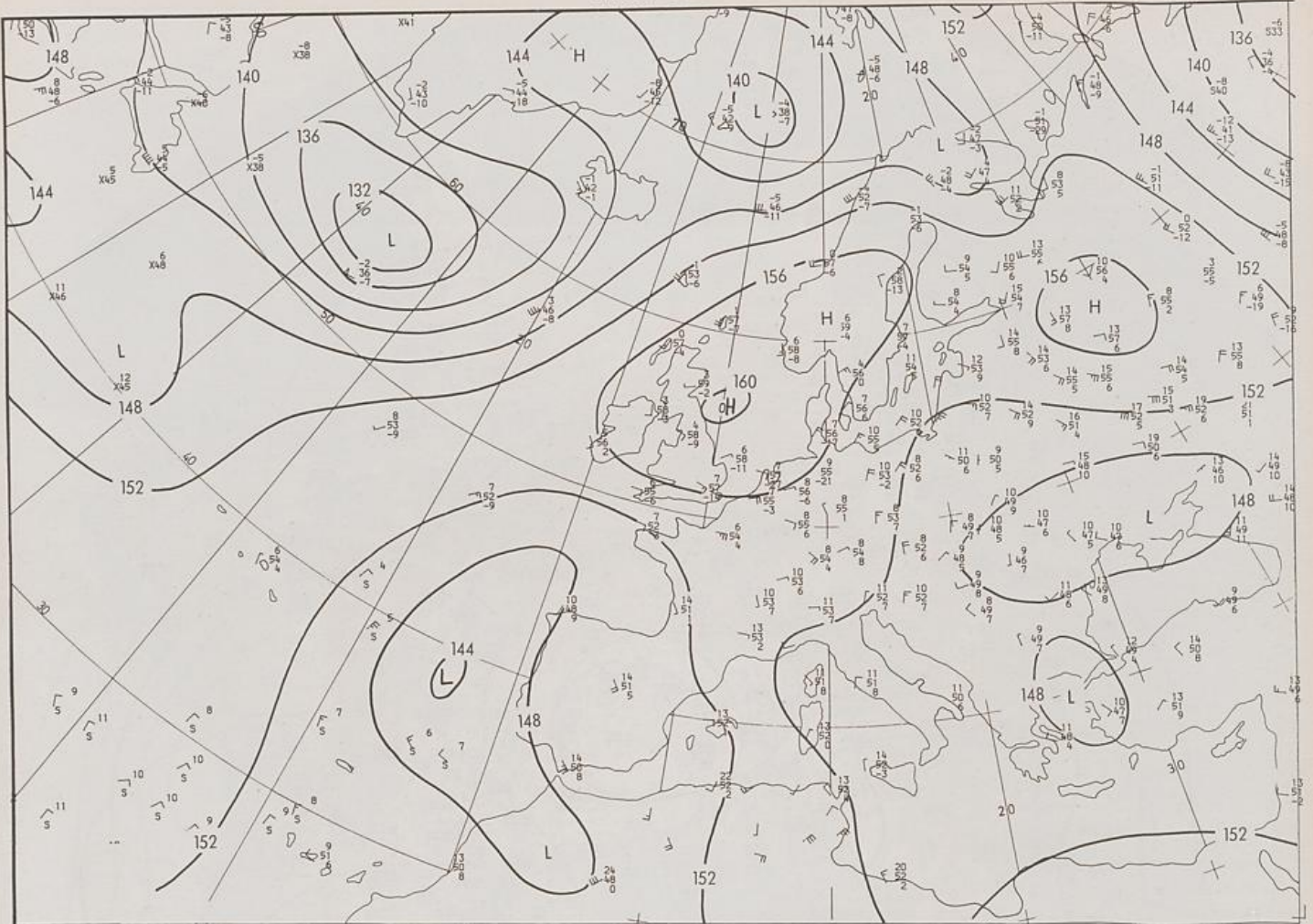
850 hPa 00 UTC
