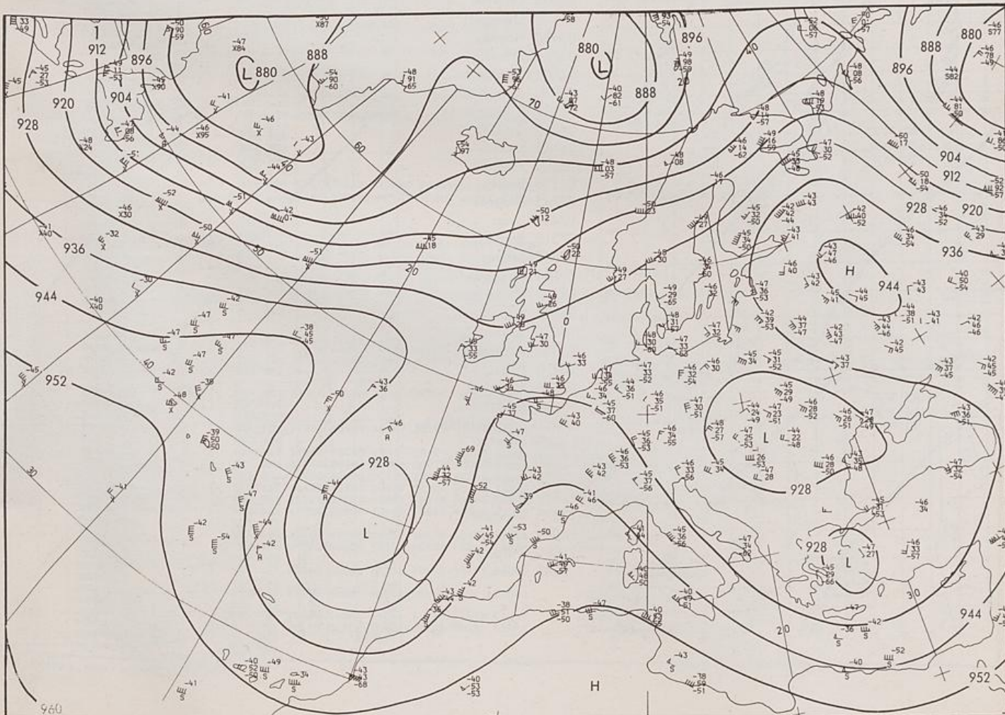
300 hPa 00 UTC
