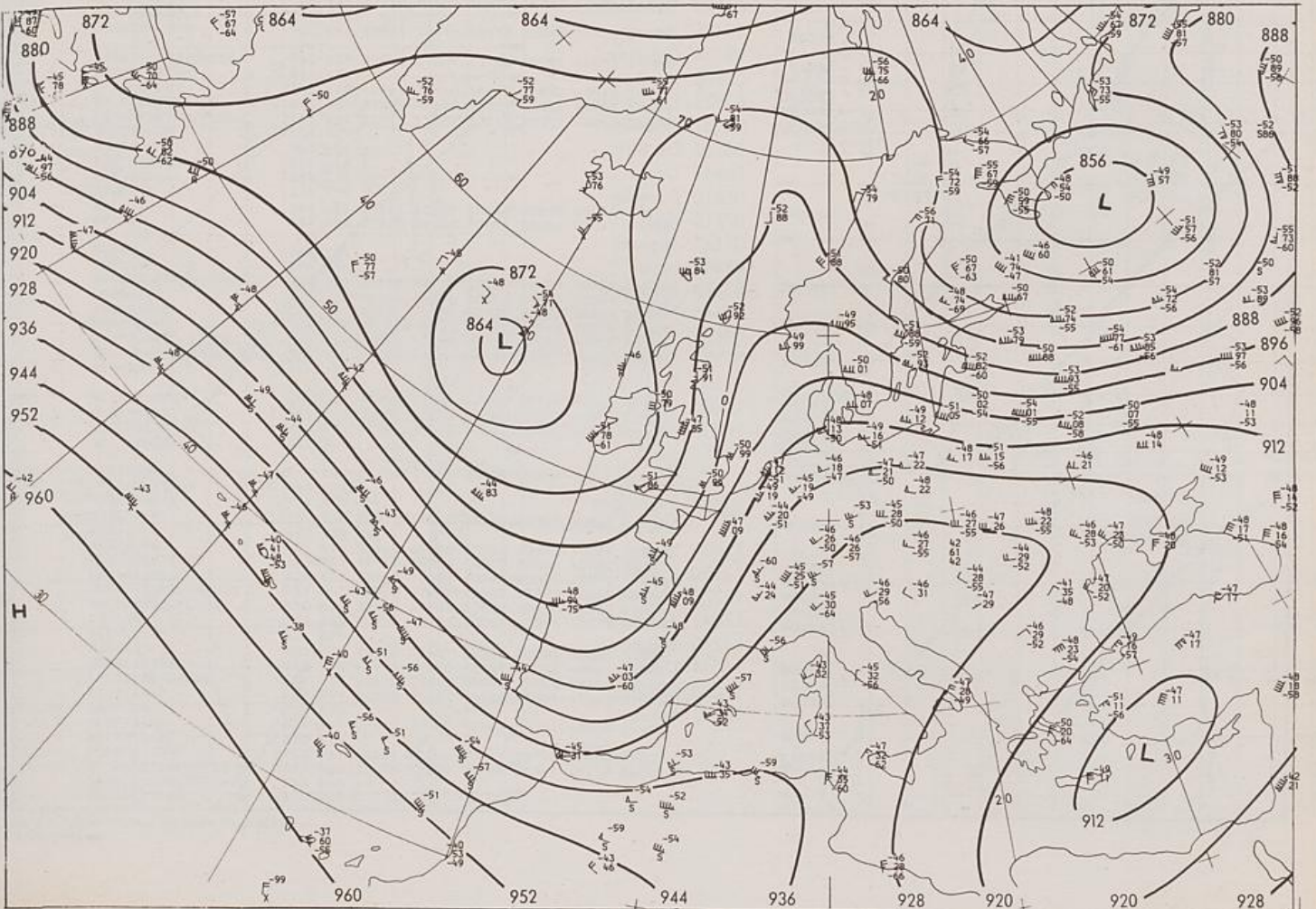
300 hPa 00 UTC
