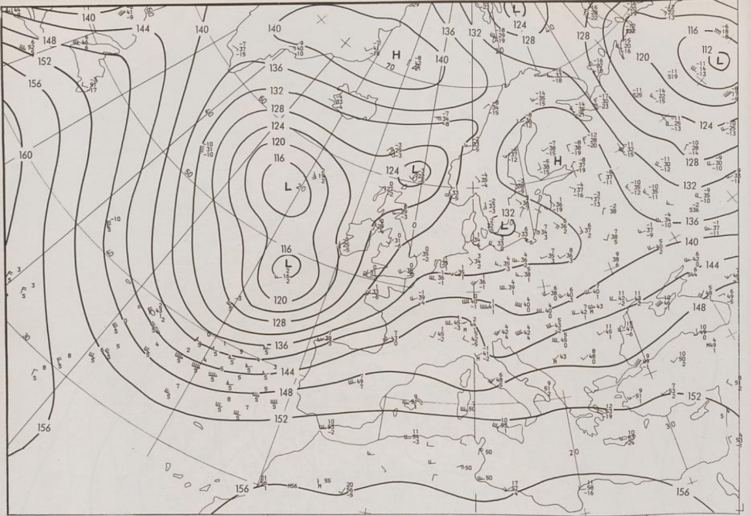
850 hPa 00 UTC
