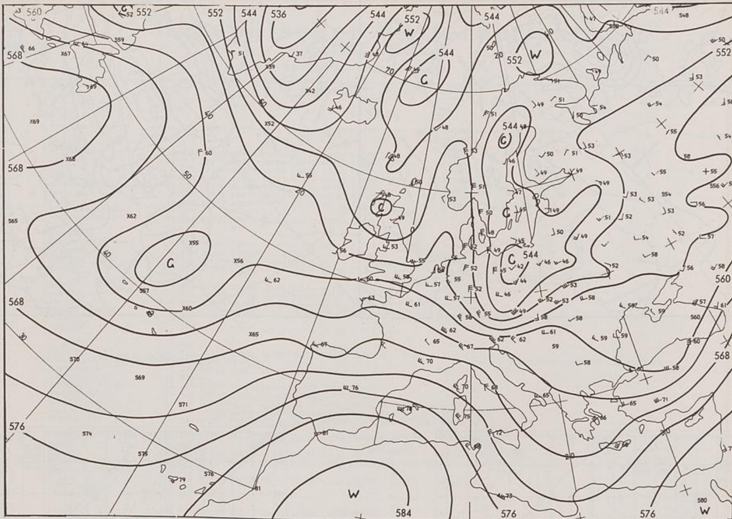
500/1000 hPa 00 UTC
