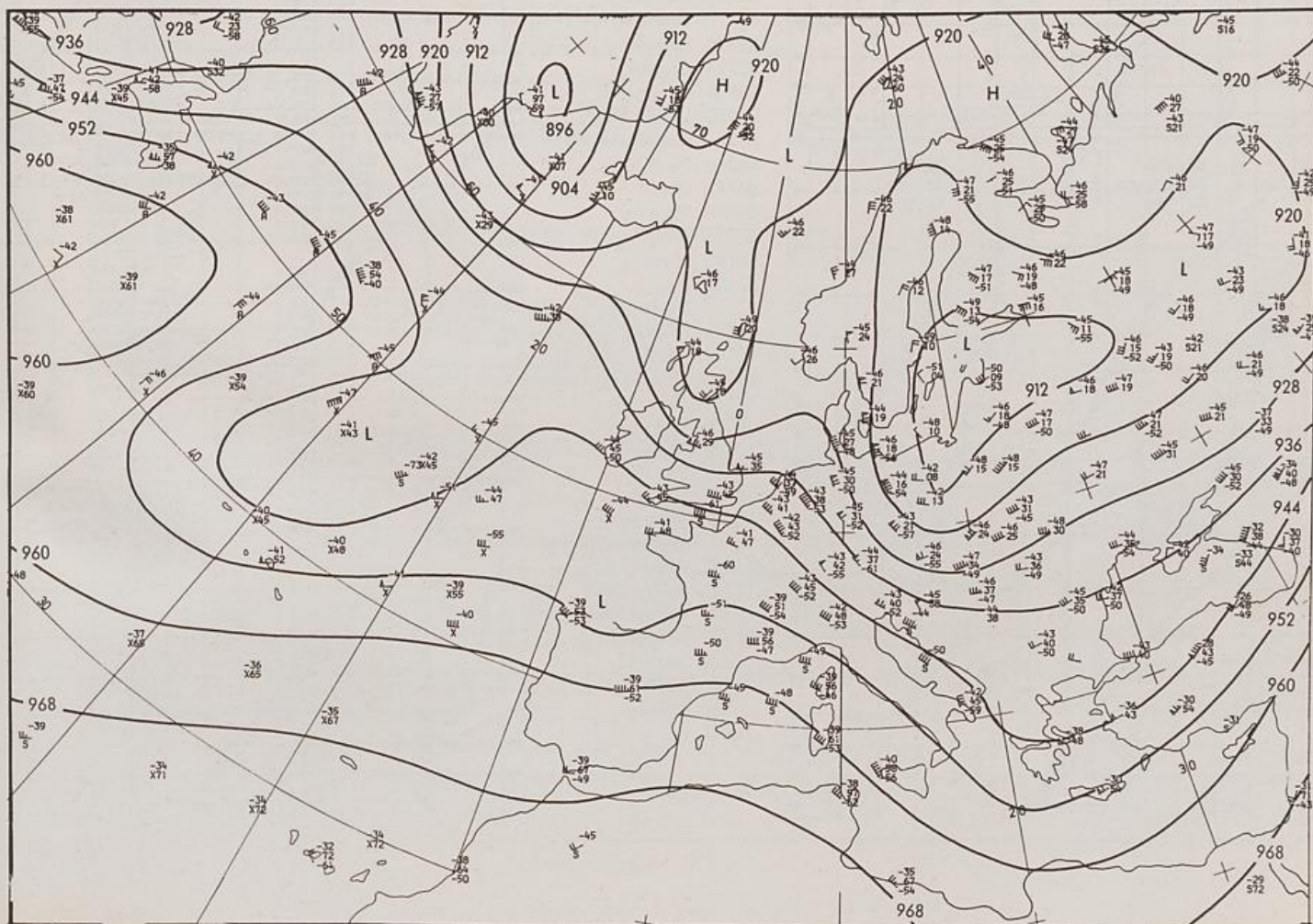
300 hPa 00 UTC
