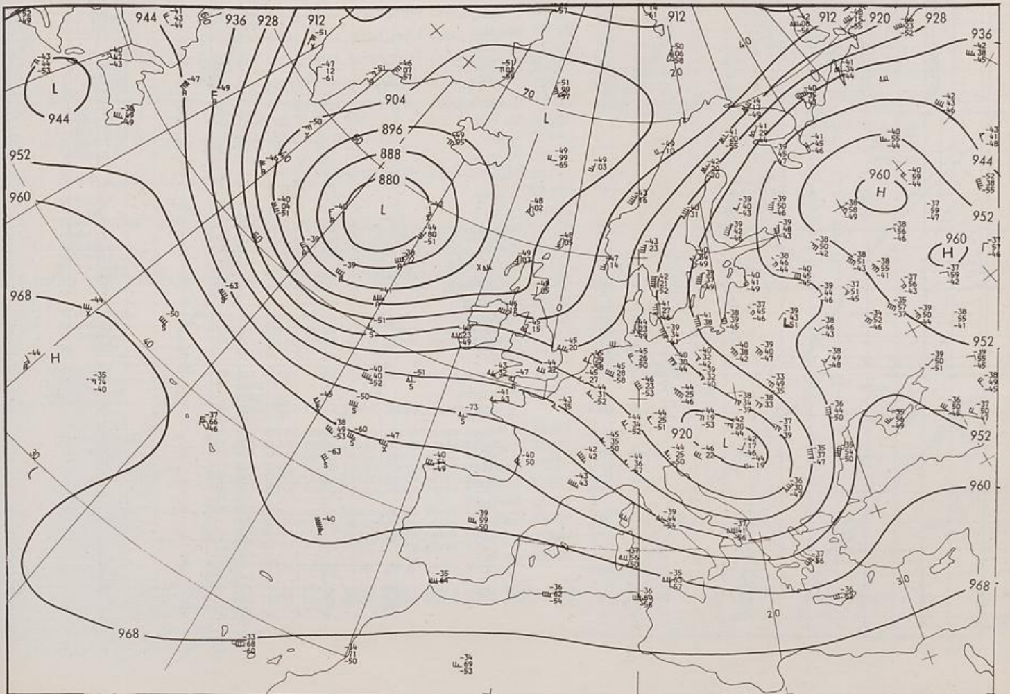
300 hPa 00 UTC
