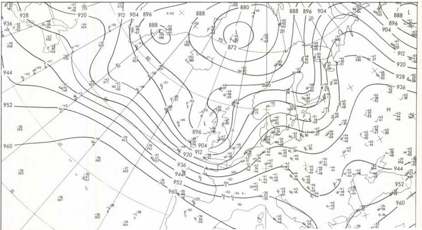
500/1000 hPa 00 UTC
