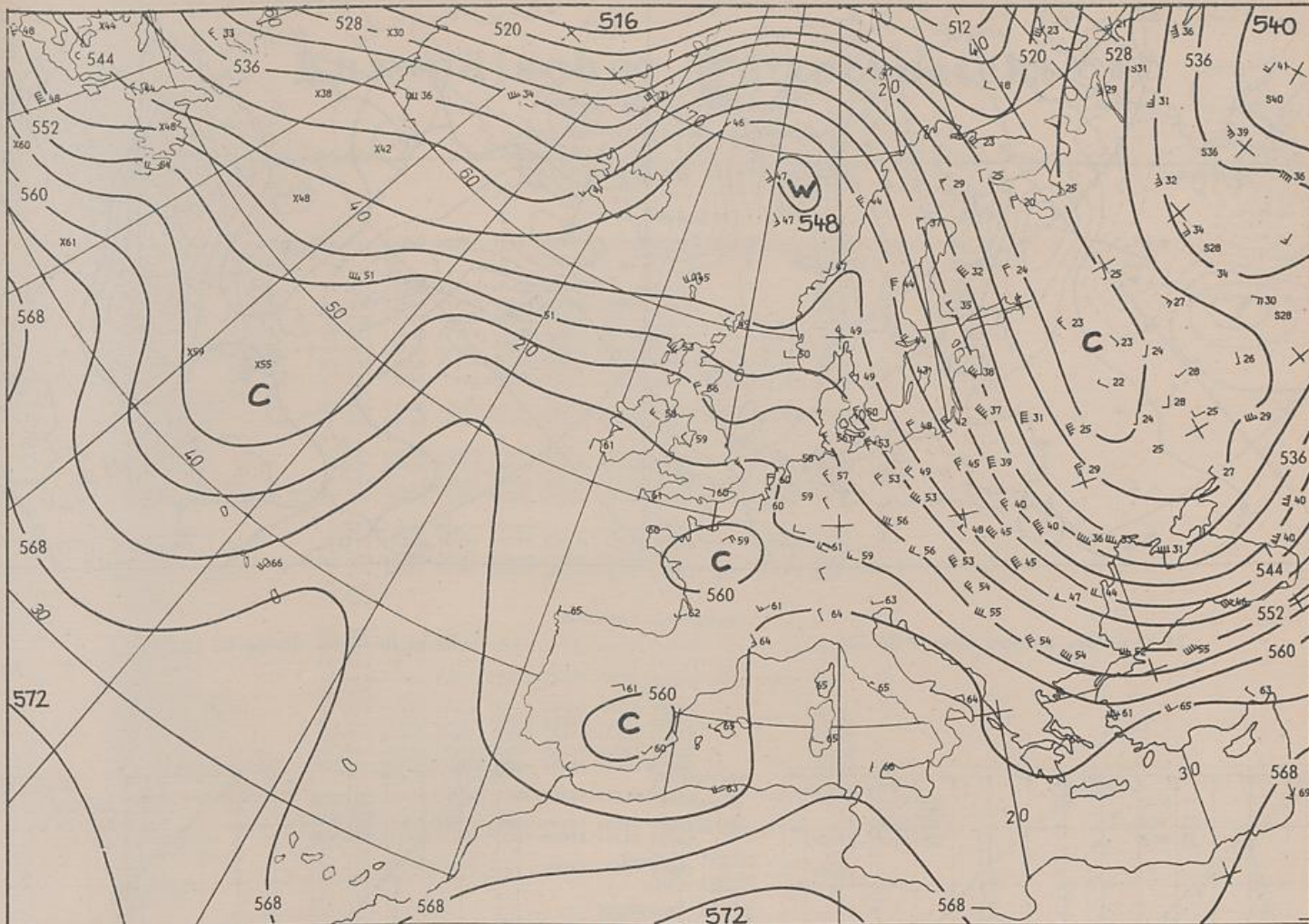
500/1000 hPa 00 UTC
