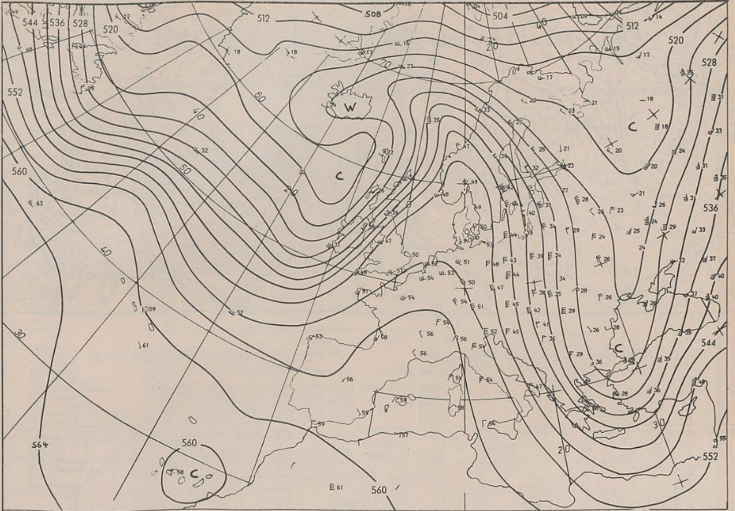
500/1000 hPa 00 UTC
