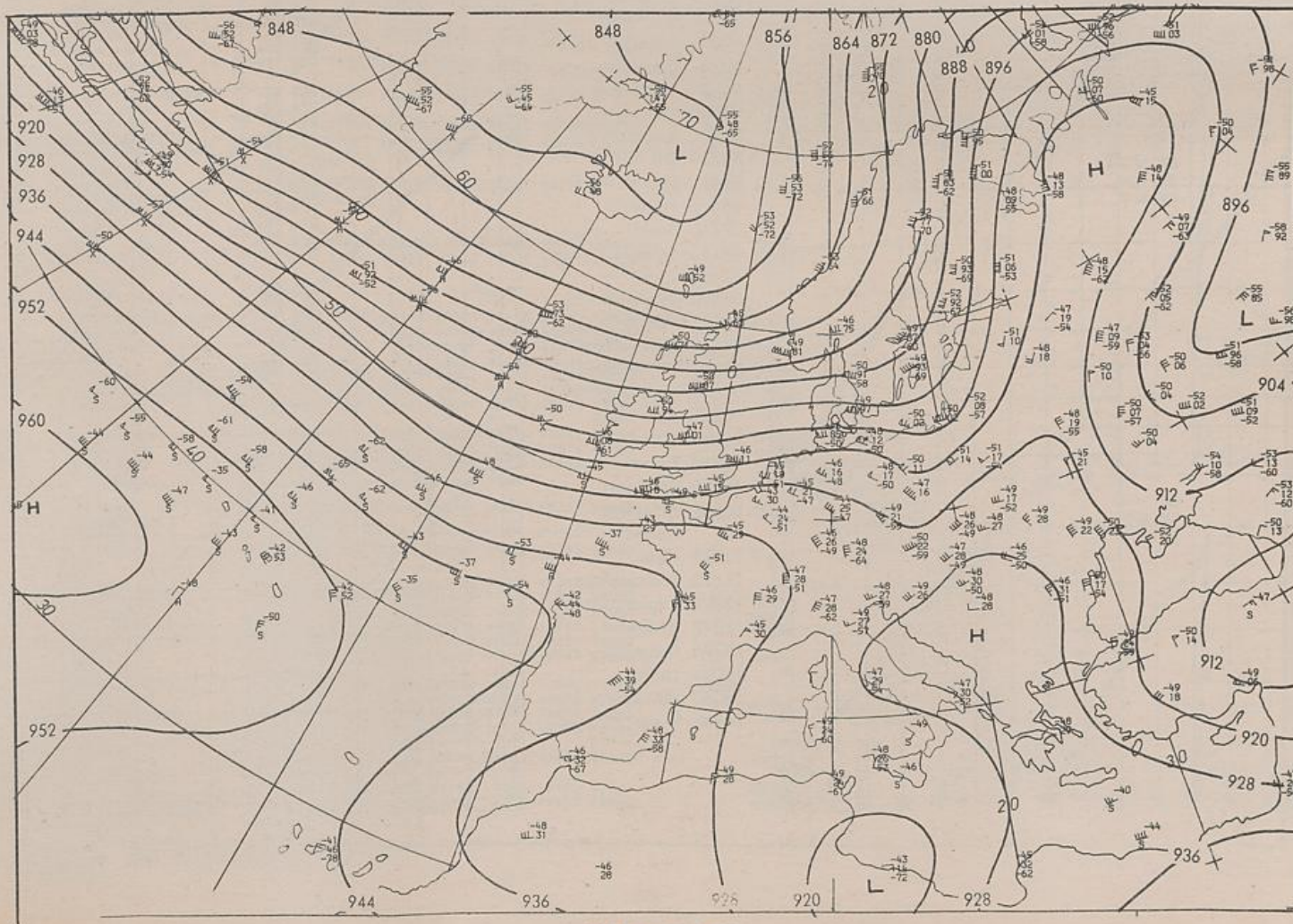
300 hPa 00 UTC
