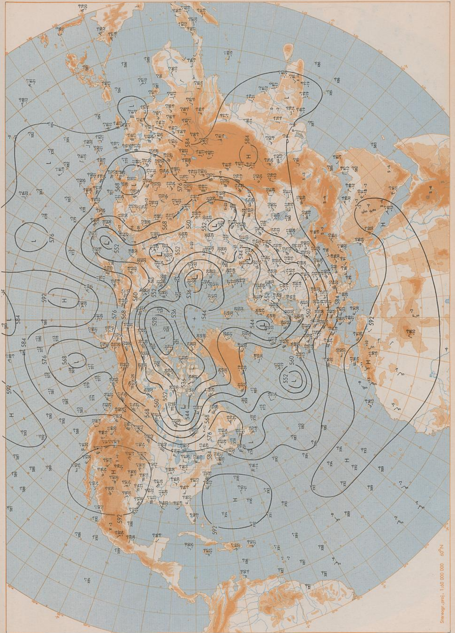
500 hPa 00 UTC
