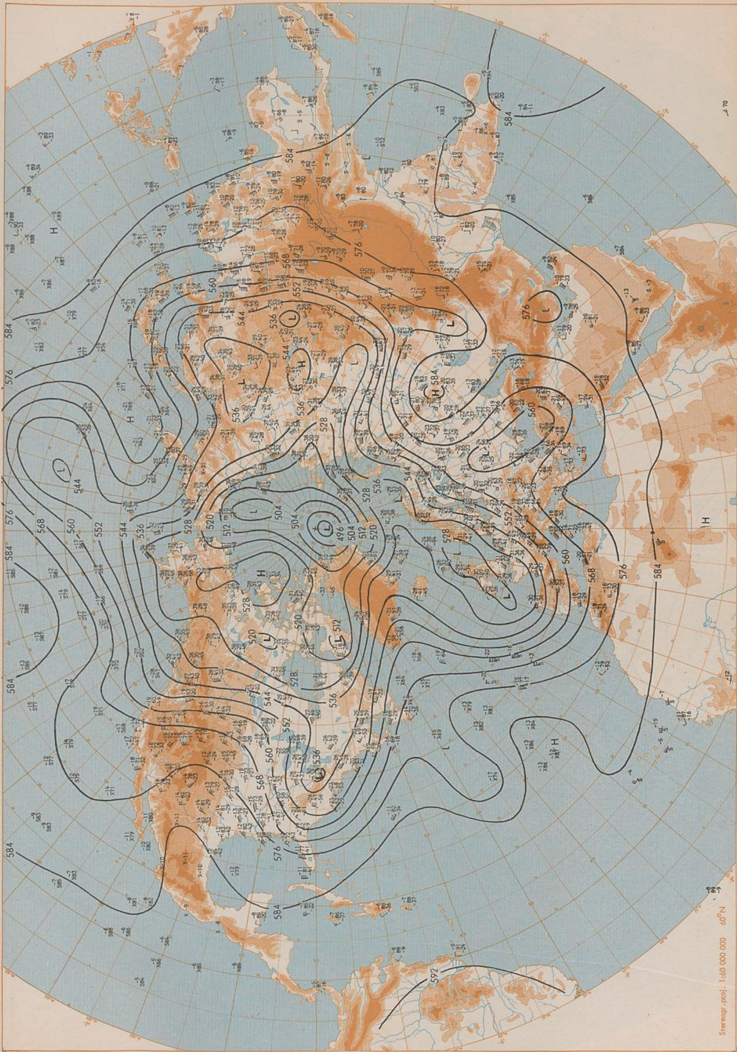
500 hPa 00 UTC
