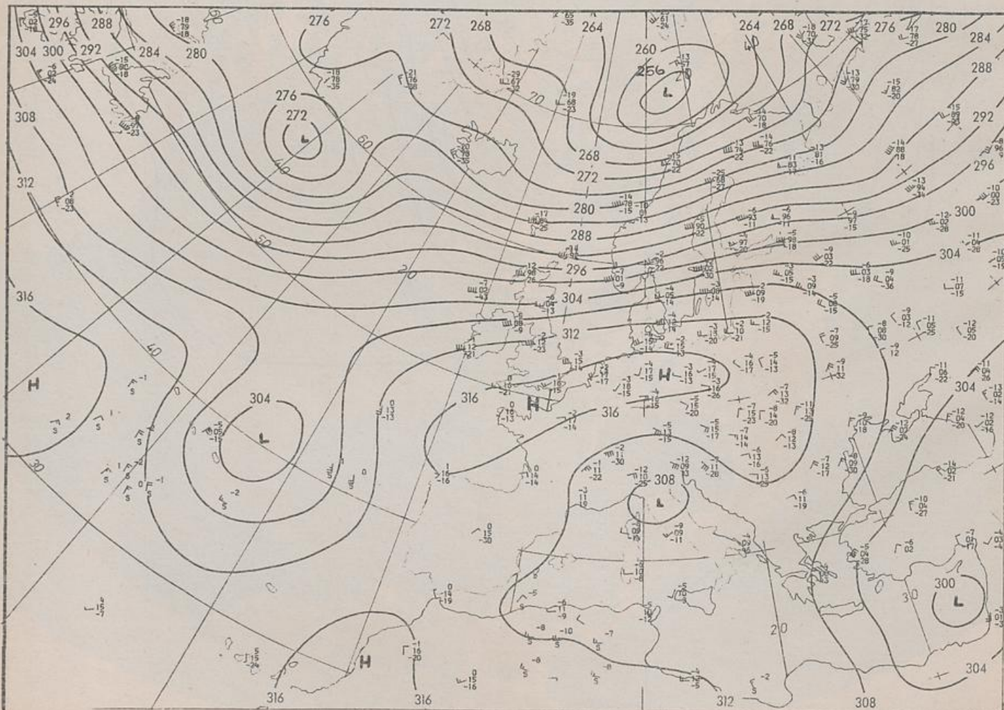
700 hPa 00 UTC
