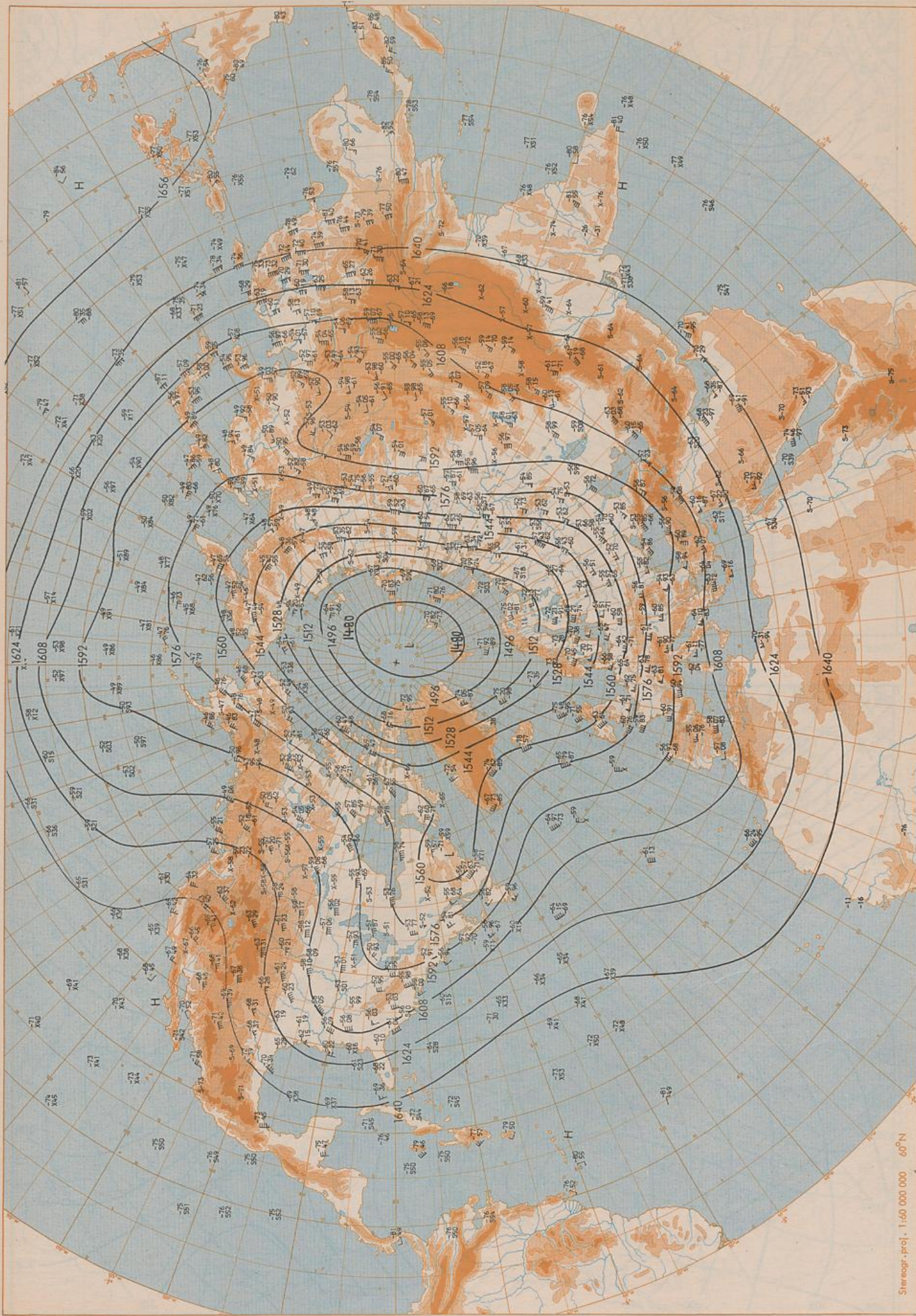
100 hPa 00 UTC
