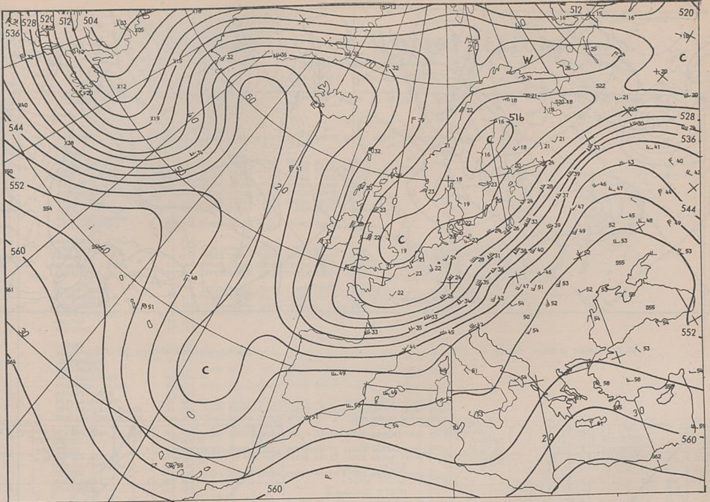
500/1000 hPa 00 UTC
