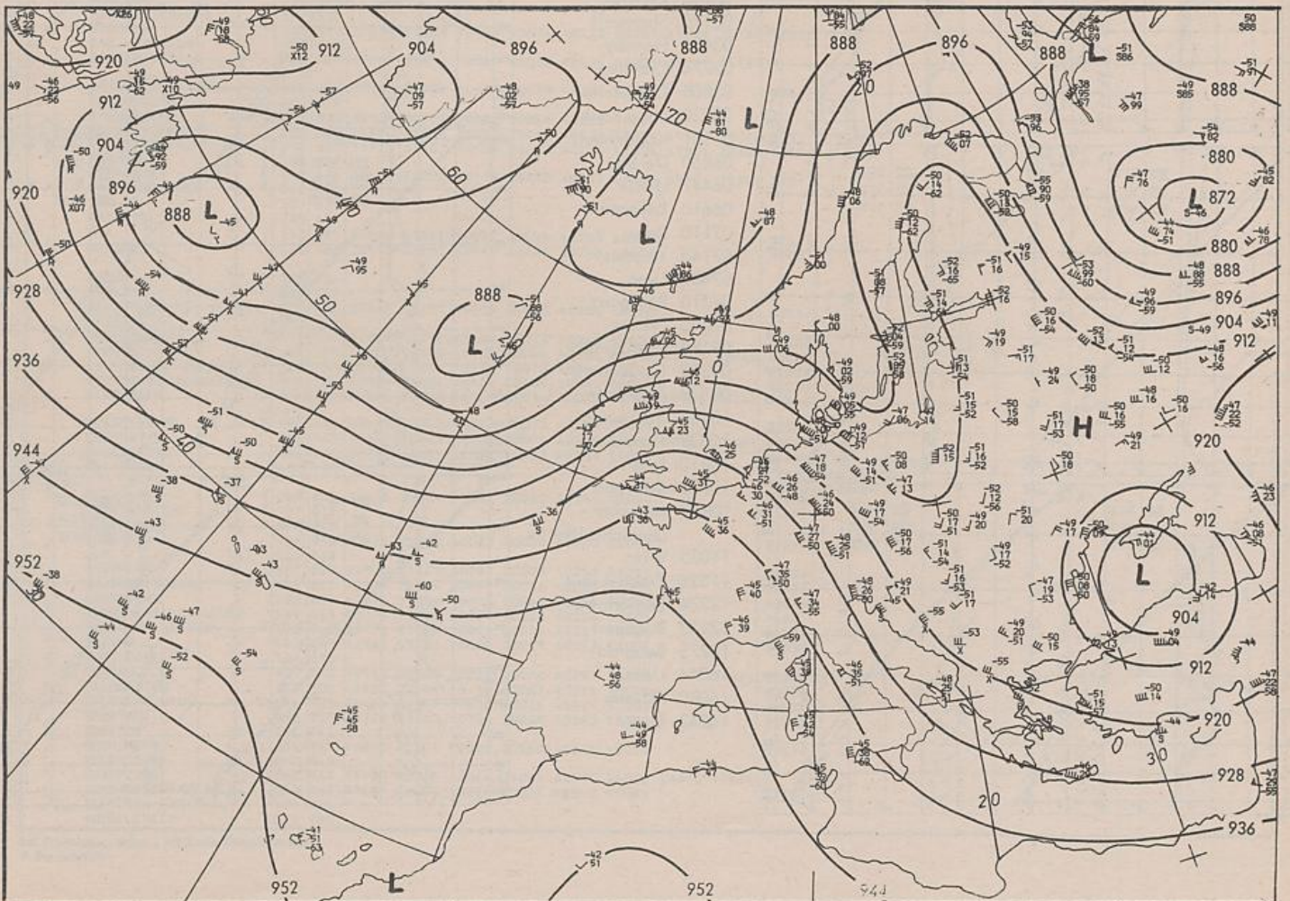
300 hPa 00 UTC
