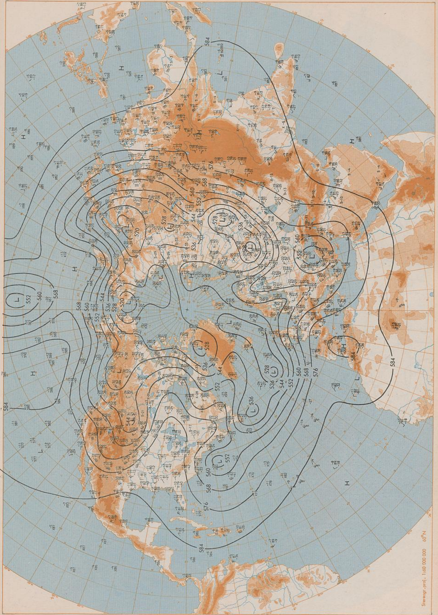
500 hPa 00 UTC
