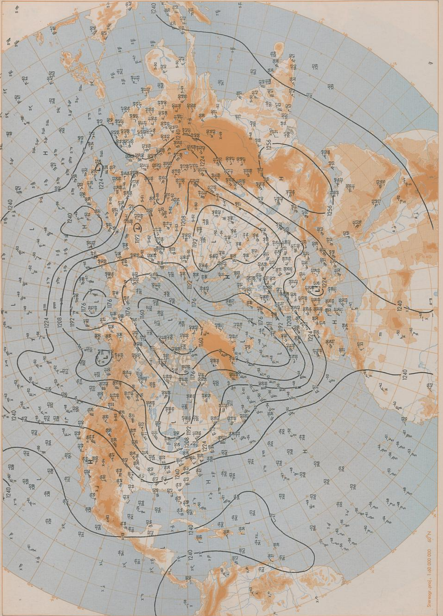
200 hPa 00 UTC
