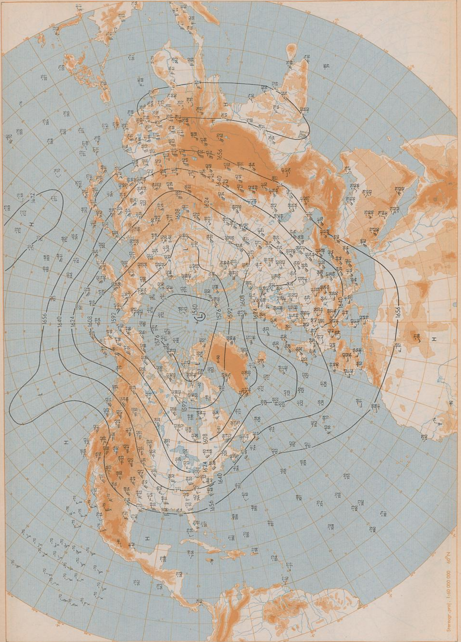
100 hPa 00 UTC
