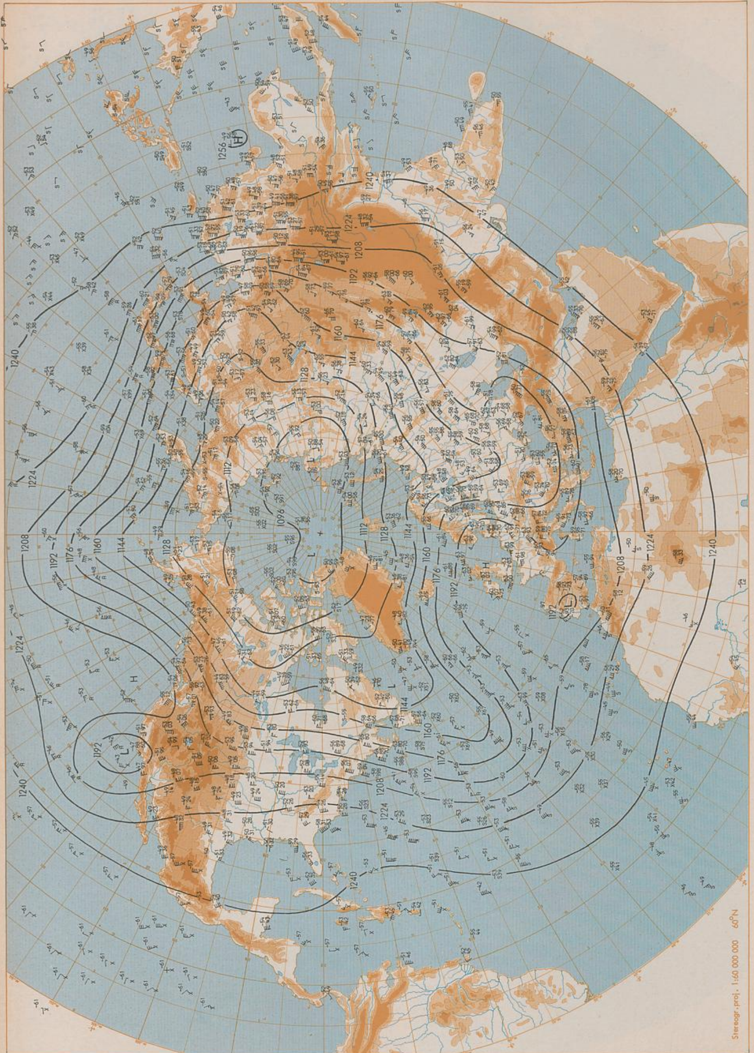
200 hPa 00 UTC
