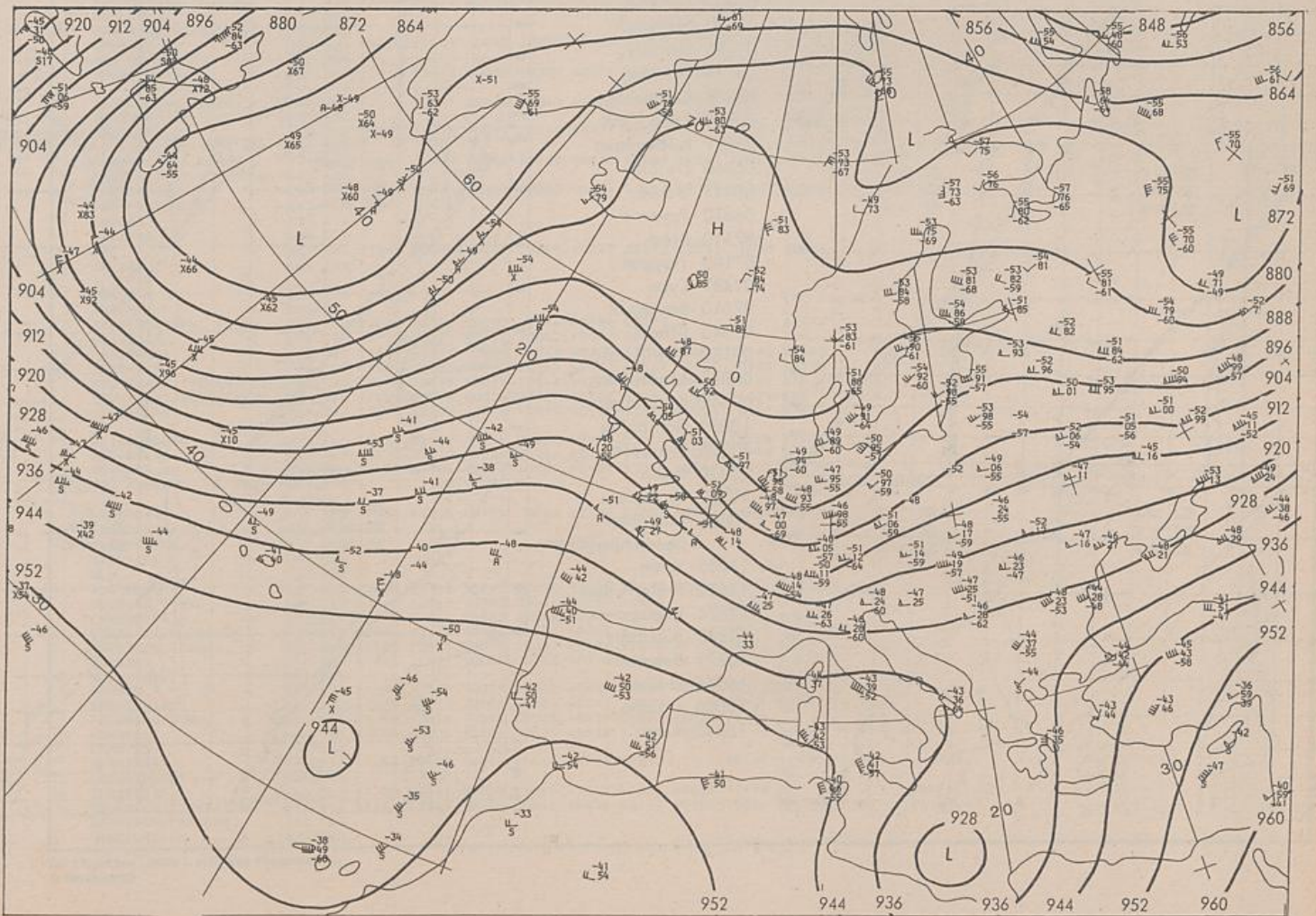
500/1000 hPa 00 UTC
