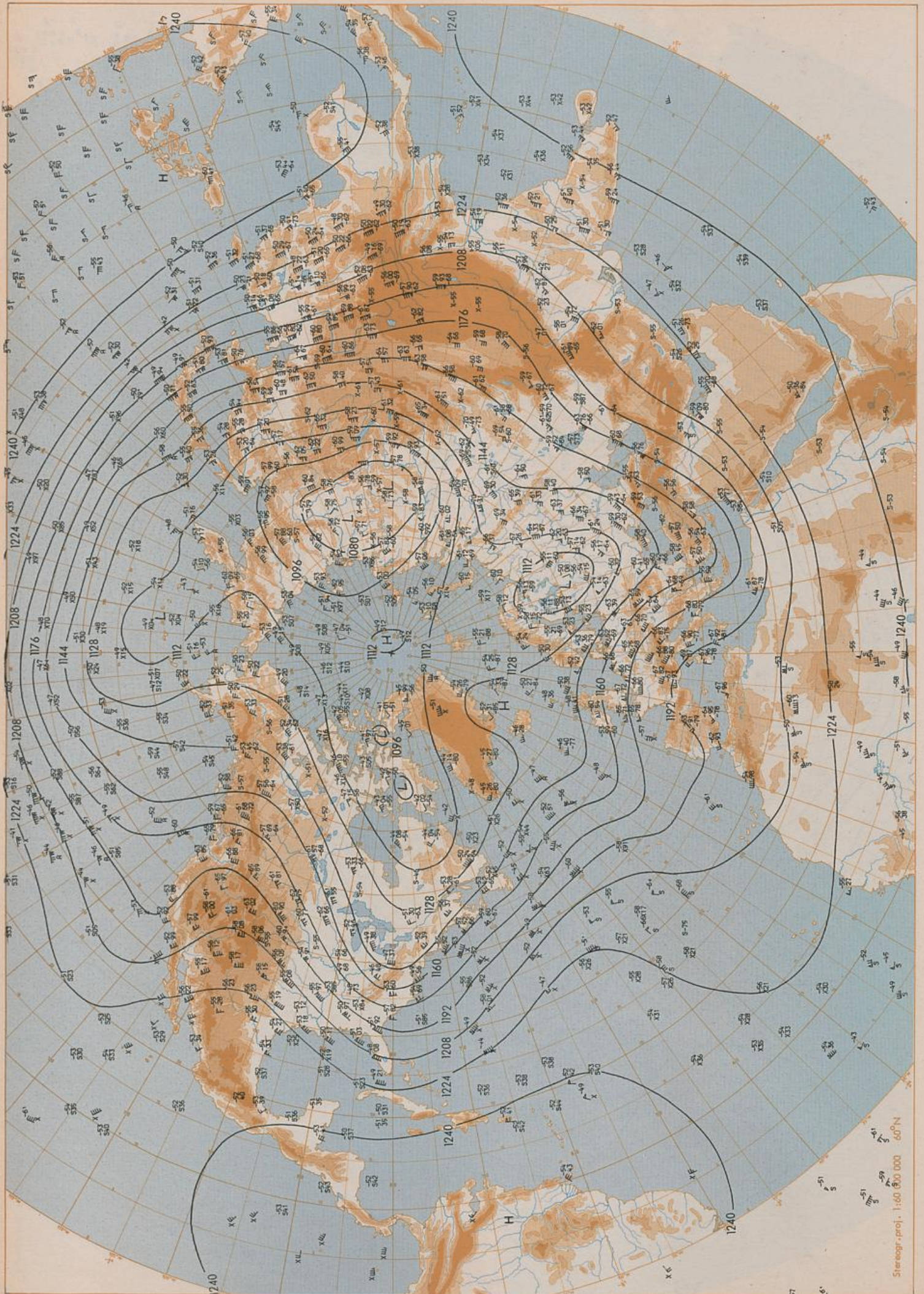
200 hPa 00 UTC
