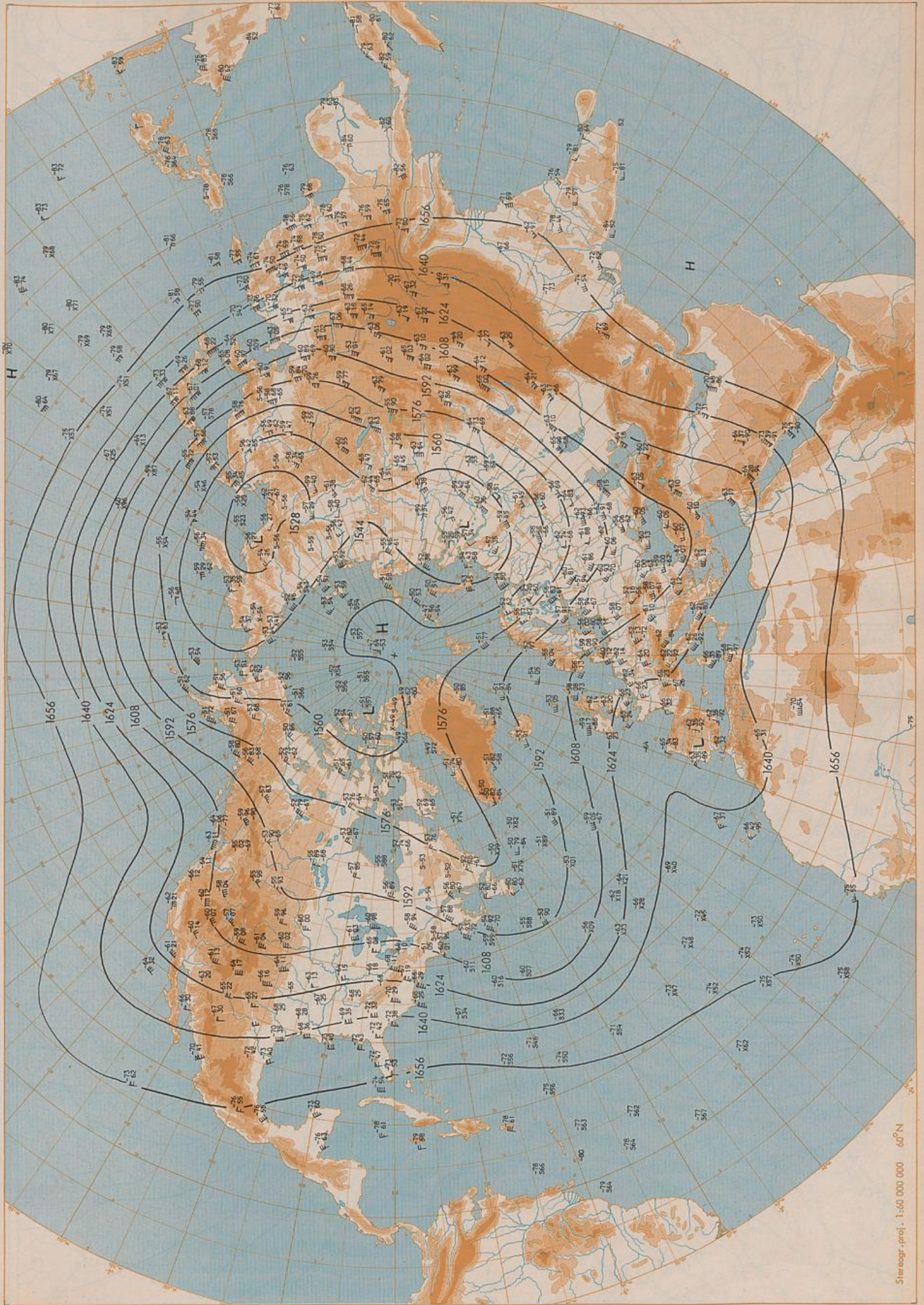
100 hPa 00 UTC
