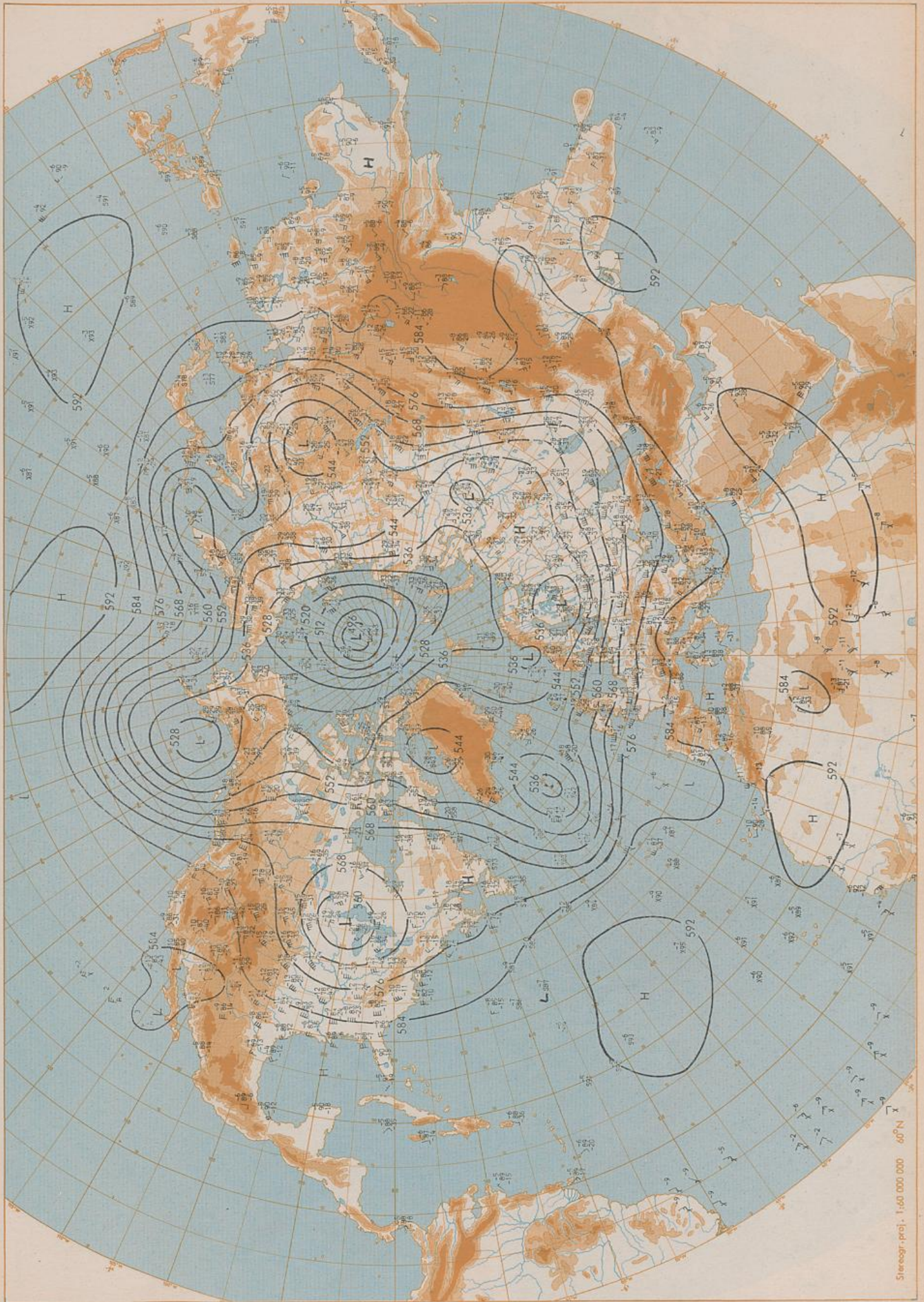
500 hPa 00 UTC
