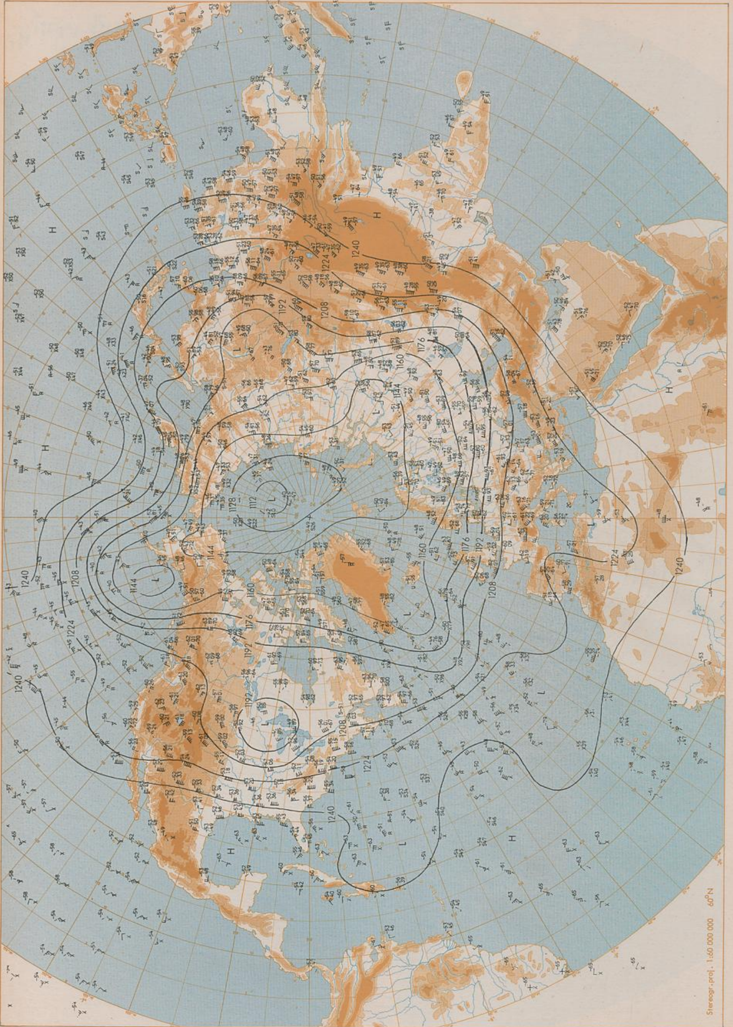
200 hPa 00 UTC
