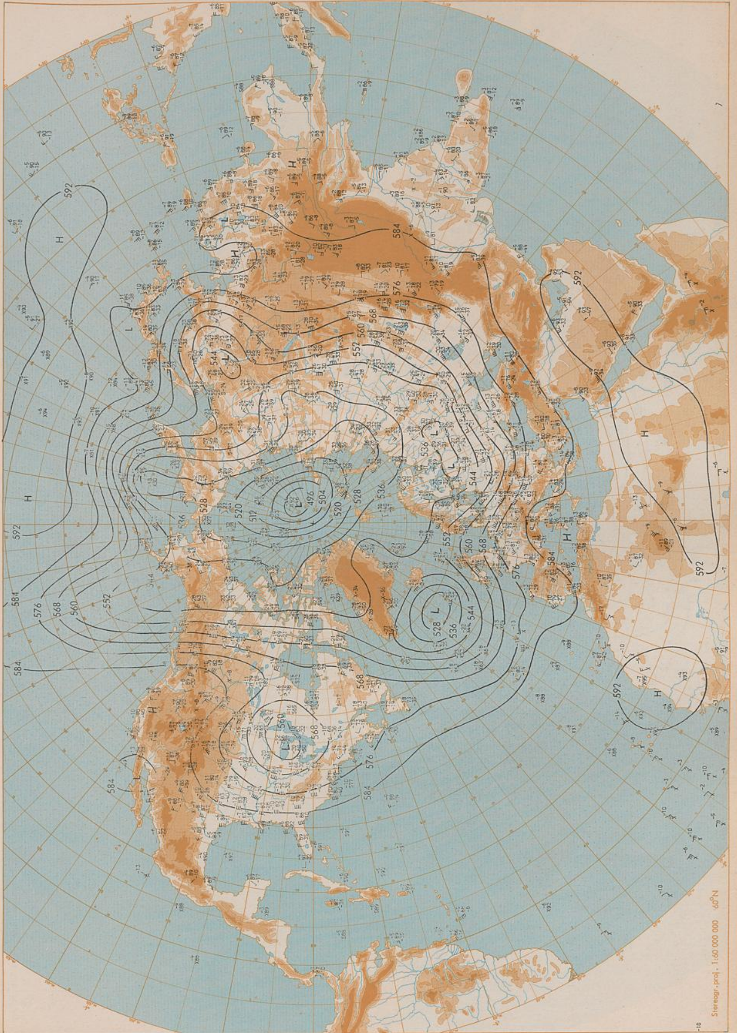
500 hPa 00 UTC
