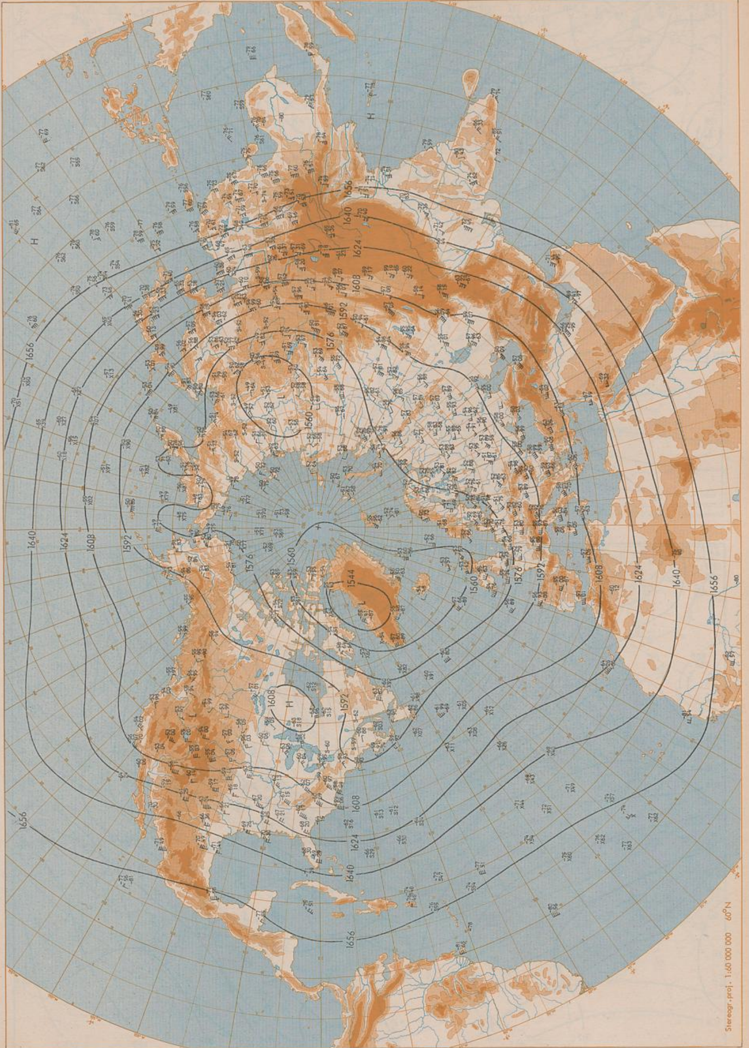
100 hPa 00 UTC
