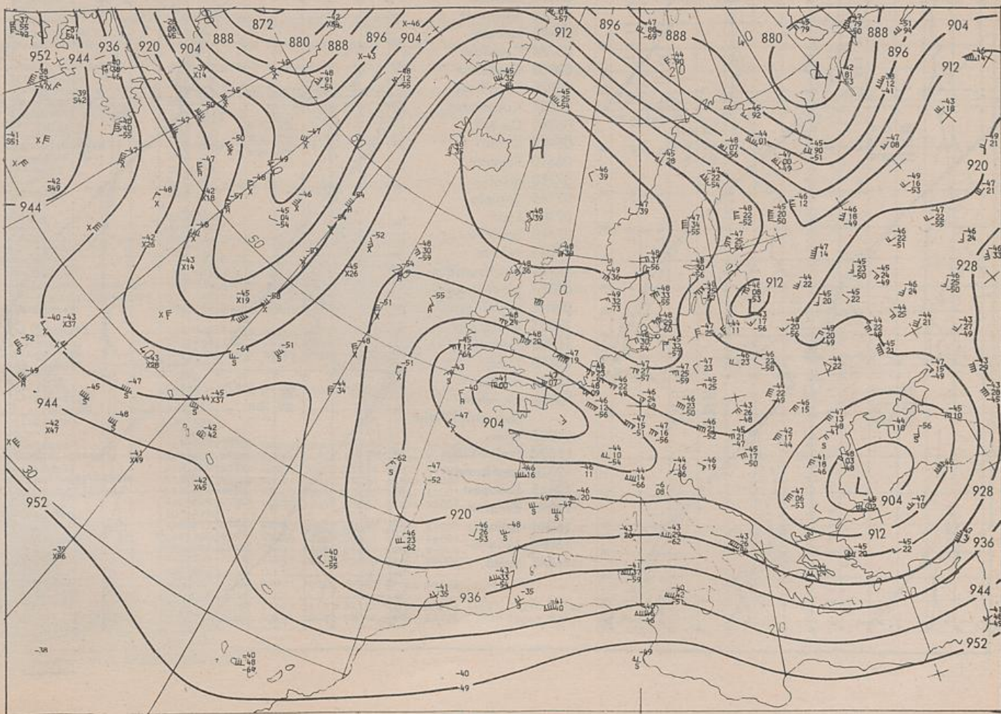
300 hPa 00 UTC
