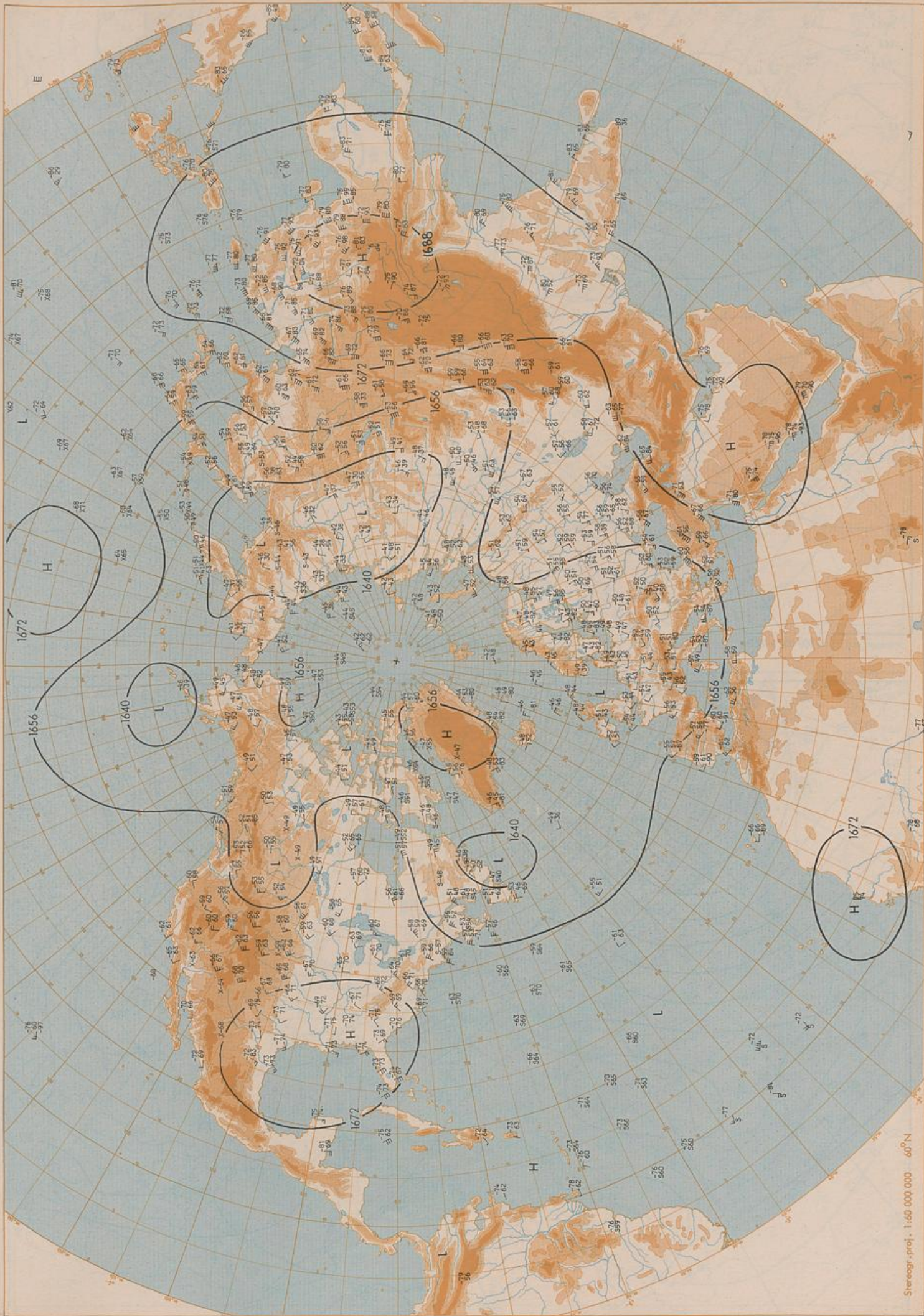
100 hPa 00 UTC
