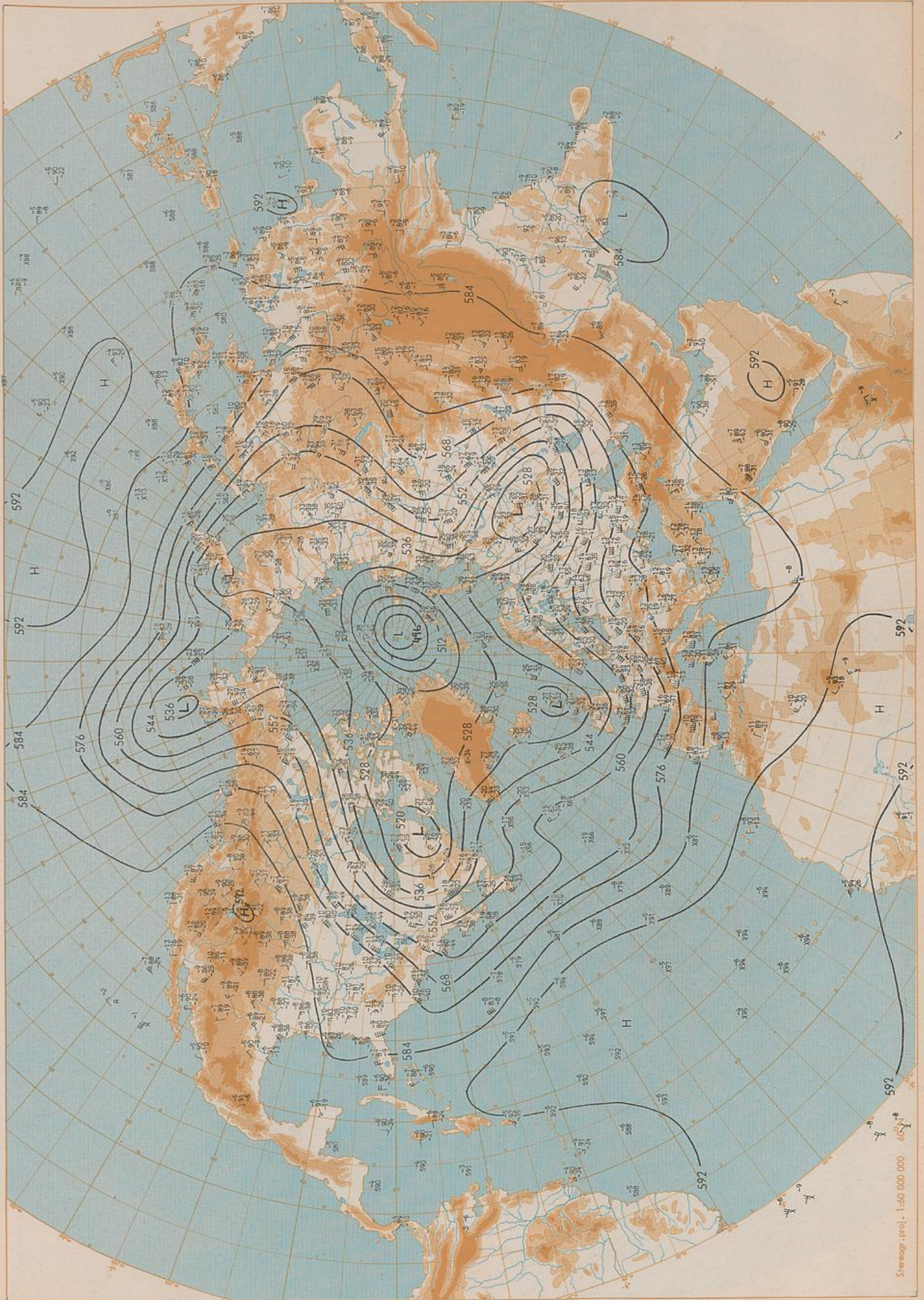
500 hPa 00 UTC
