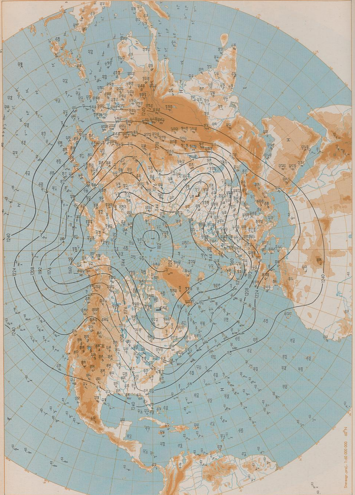
200 hPa 00 UTC
