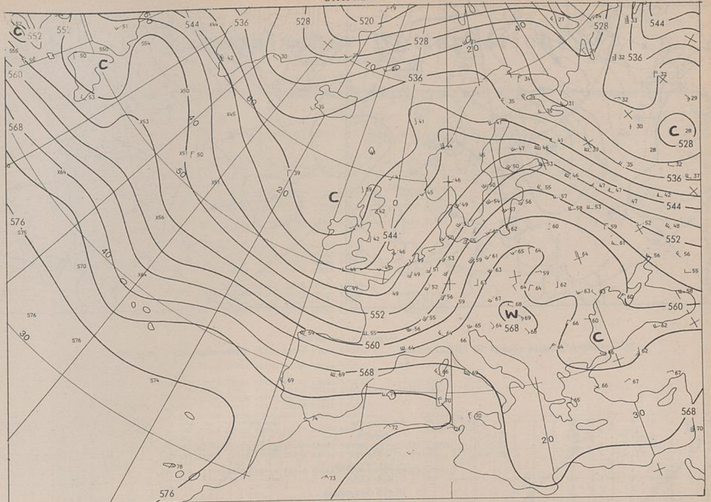
500/1000 hPa 00 UTC
