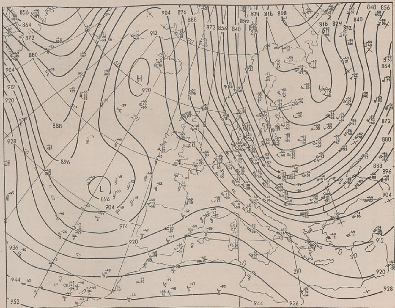
300 hPa 00 UTC
