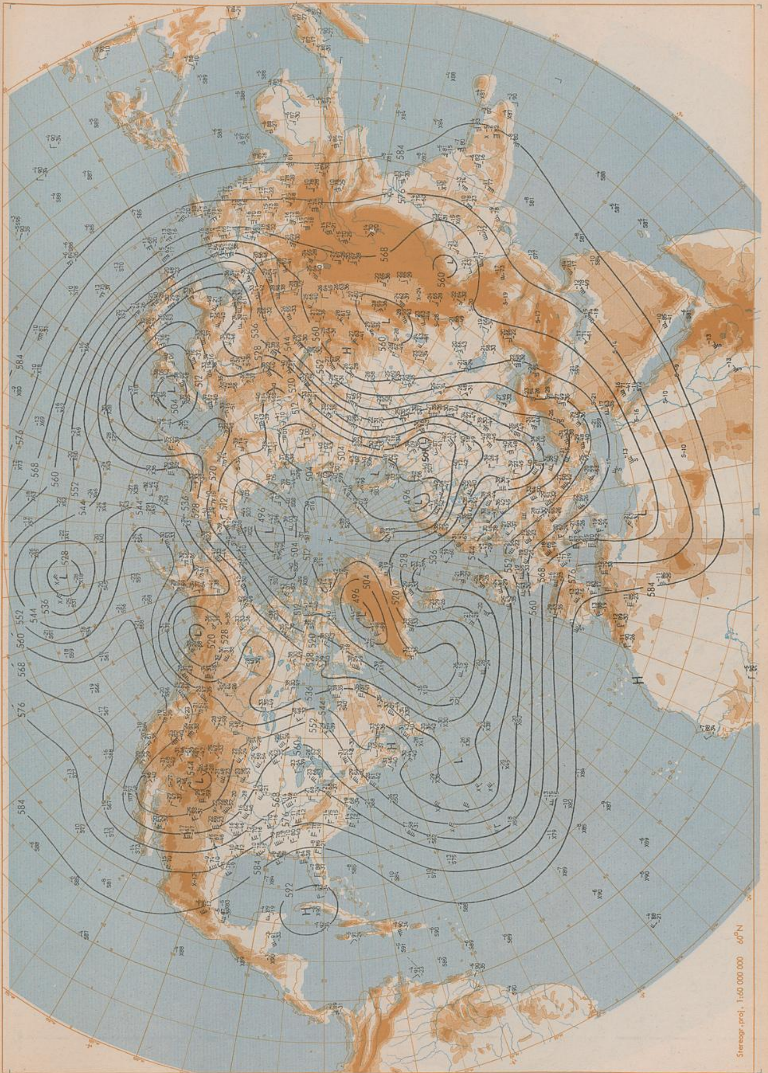
500 hPa 00 UTC
