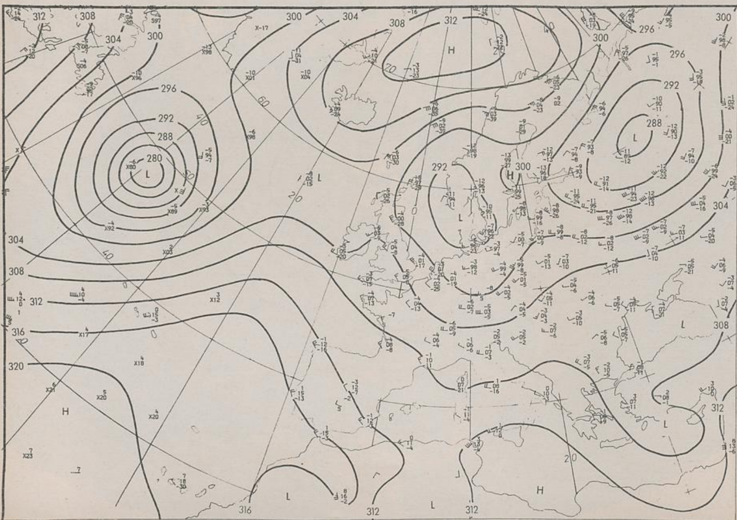
700 hPa 00 UTC
