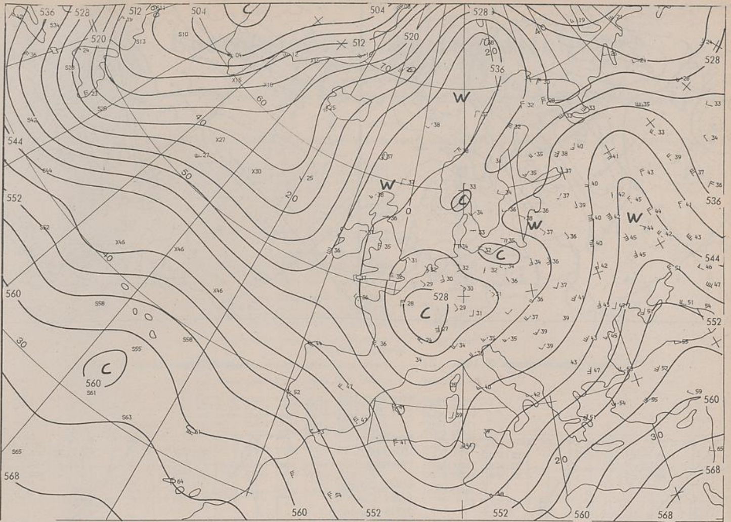
500/1000 hPa 00 UTC
