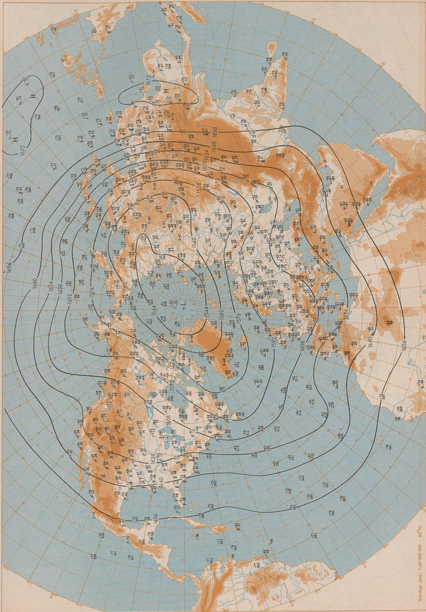
100 hPa 00 UTC
