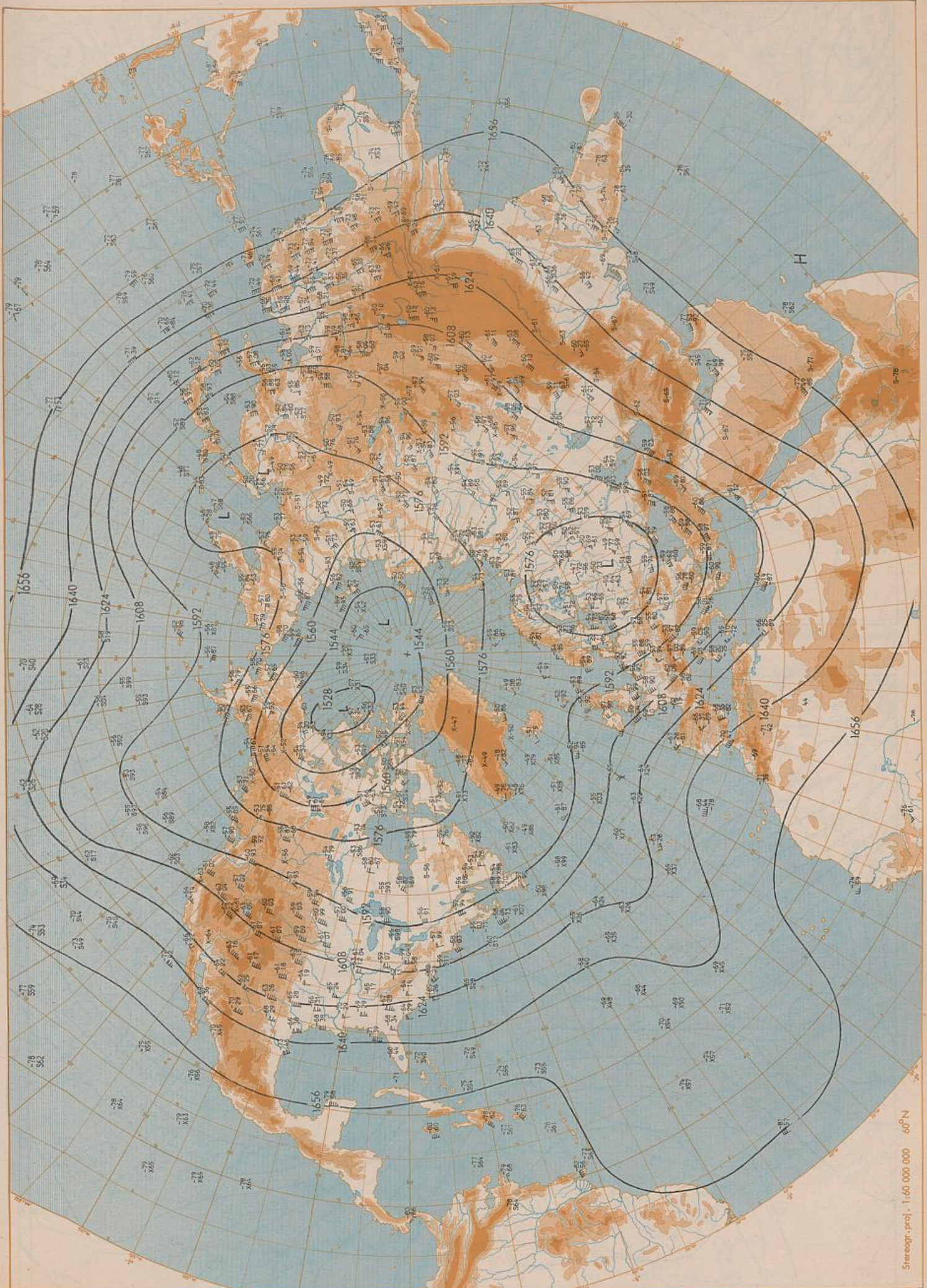
100 hPa 00 UTC
