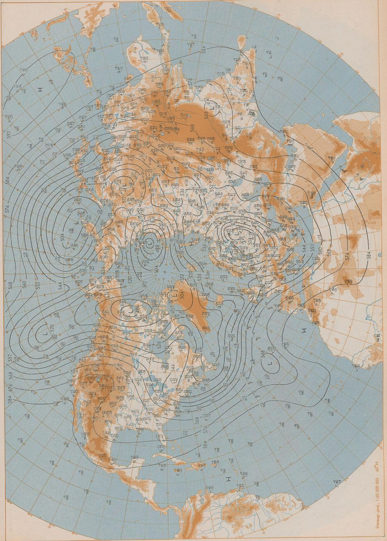
500 hPa 00 UTC
