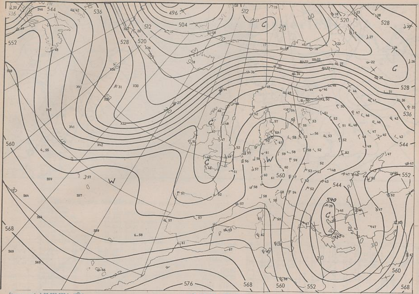
500/1000 hPa 00 UTC
