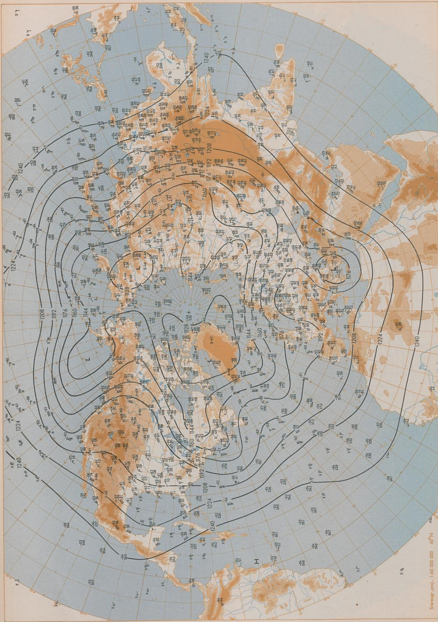
200 hPa 00 UTC
