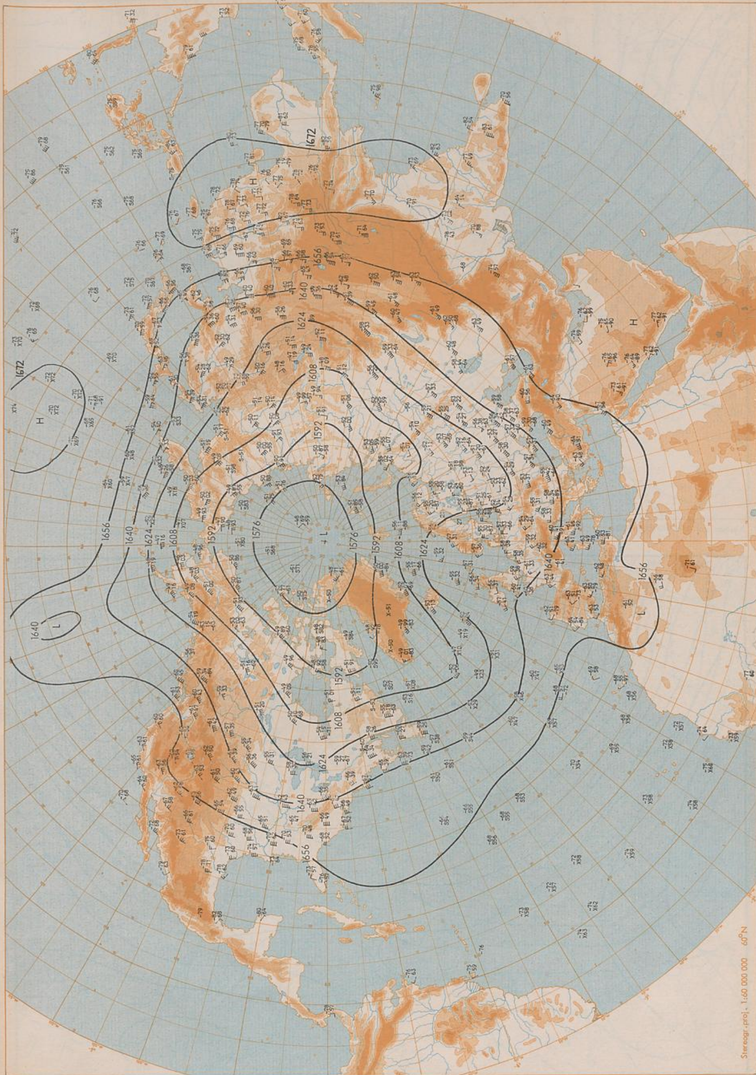
100 hPa 00 UTC
