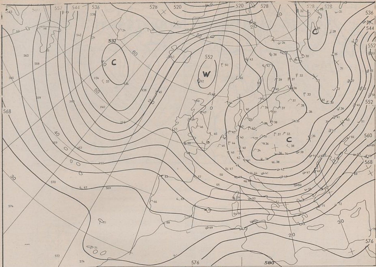
500/1000 hPa 00 UTC
